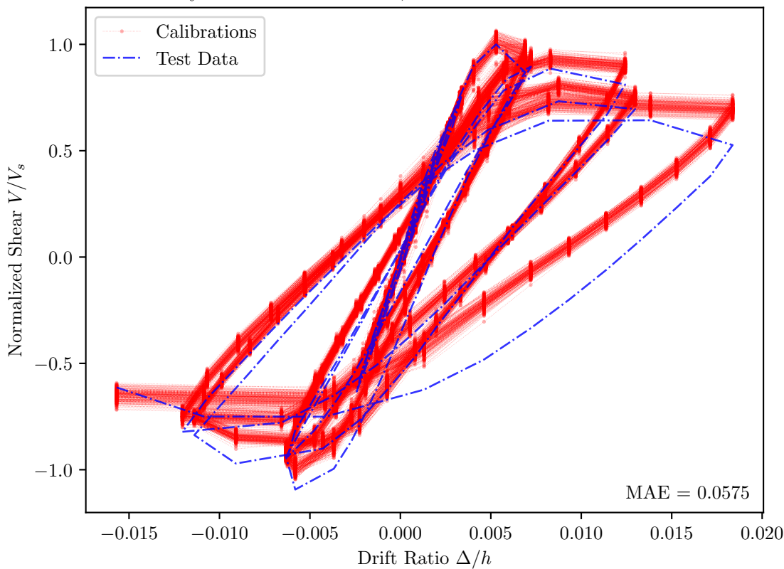
Bayrak and Sheikh 1996, AS-7HT — PEER Id = 163
