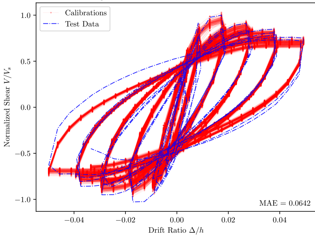
Saatcioglu and Grira 1999, BG-2 — PEER Id = 166
