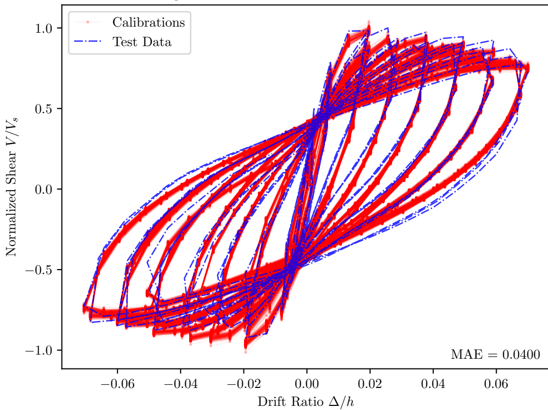
Saatcioglu and Grira 1999, BG-3 — PEER Id = 167
