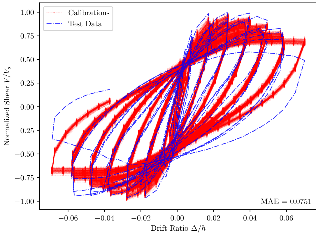
Saatcioglu and Grira 1999, BG-6 — PEER Id = 170
