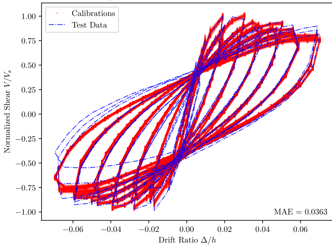
Saatcioglu and Grira 1999, BG-8 — PEER Id = 172
