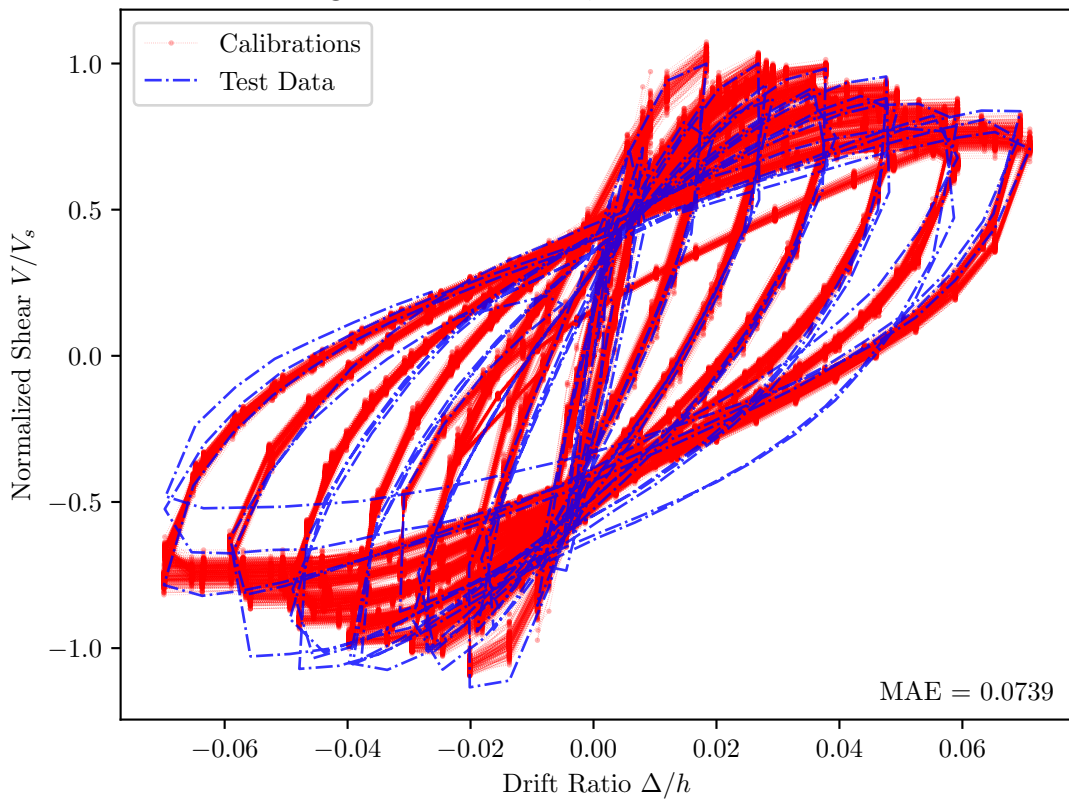
Saatcioglu and Grira 1999, BG-10 — PEER Id = 174
