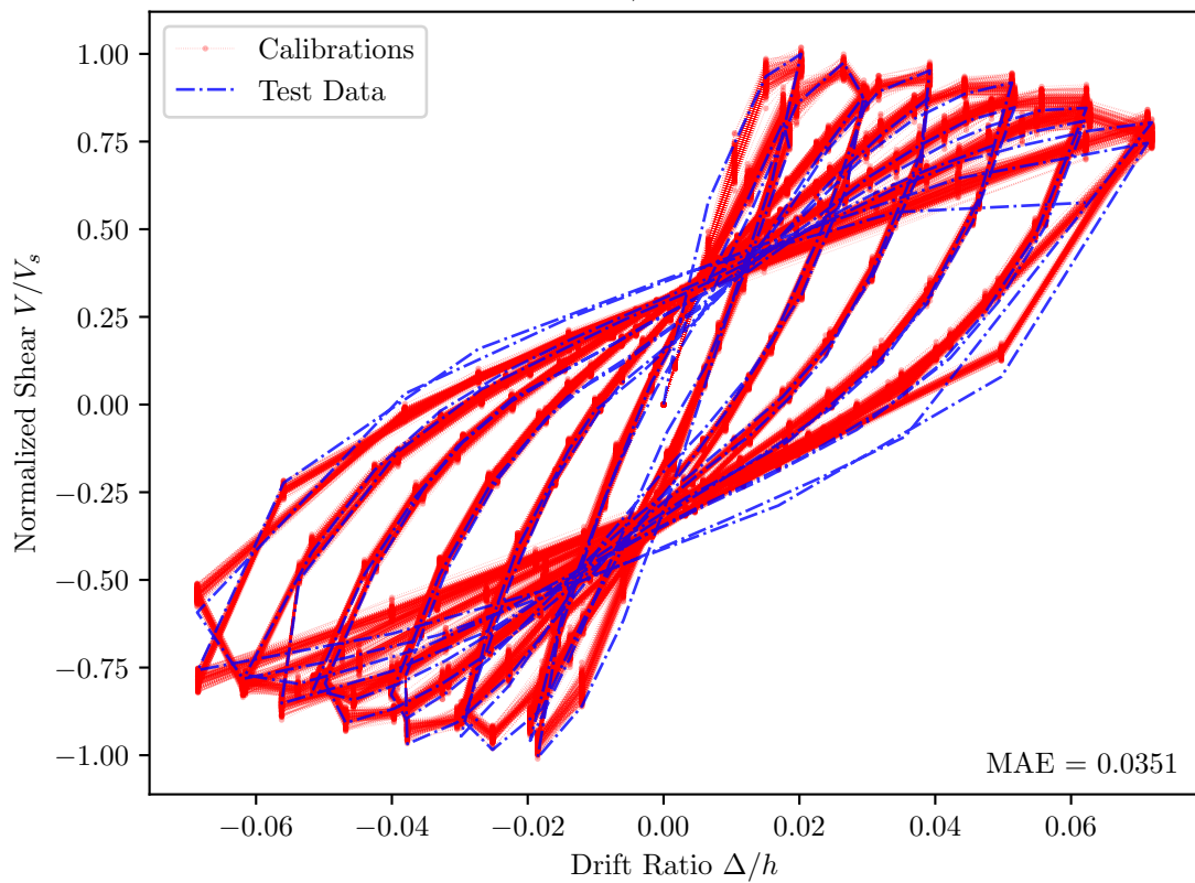
Matamoros et al. 1999,C10-05S — PEER Id = 176
