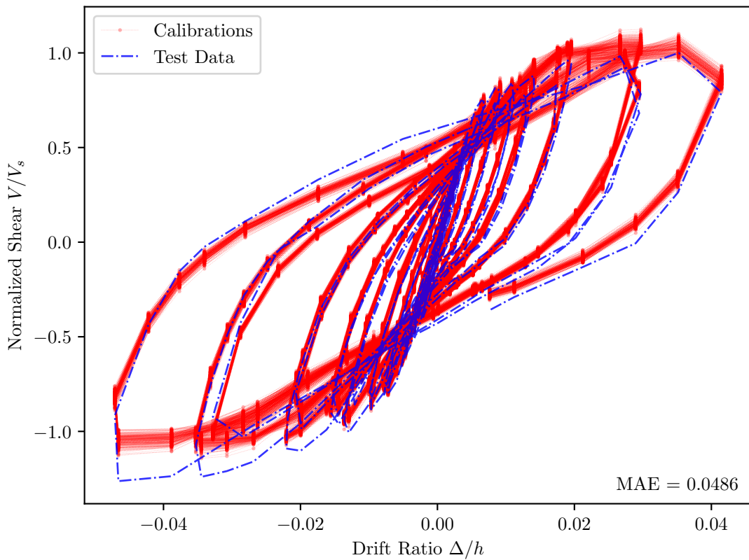
Thomsen and Wallace 1994, B1 — PEER Id = 203
