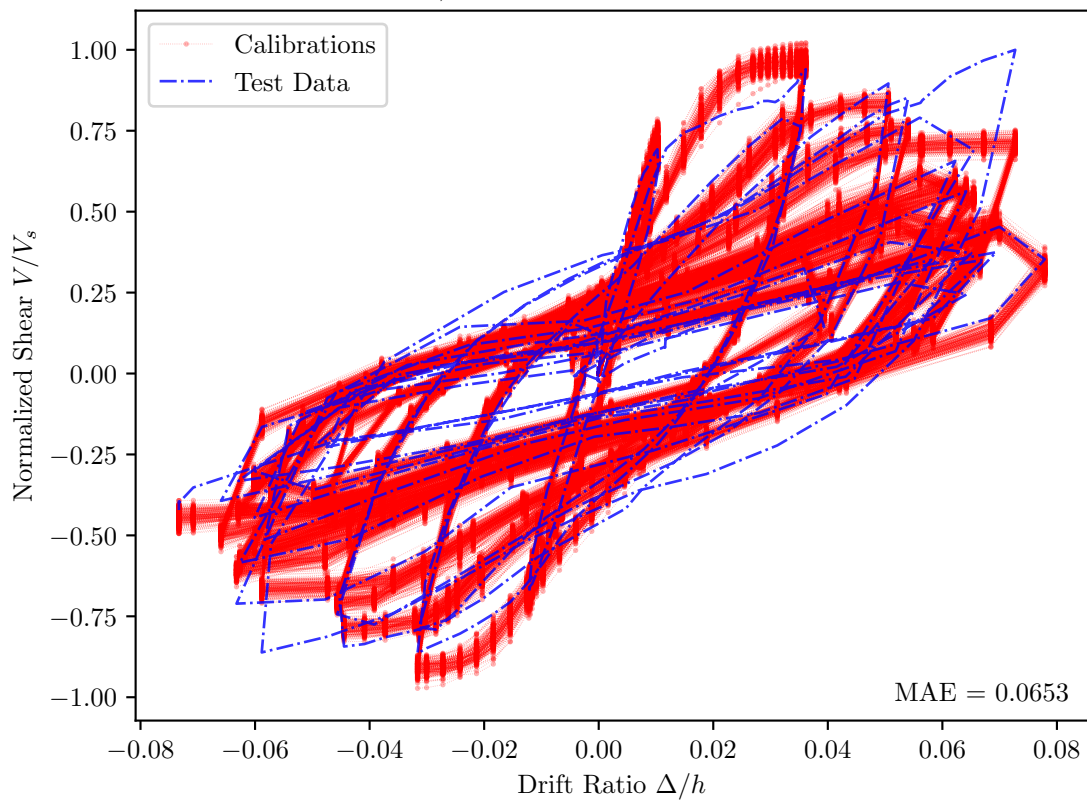
NIST, Model N3 — PEER Id = 310
