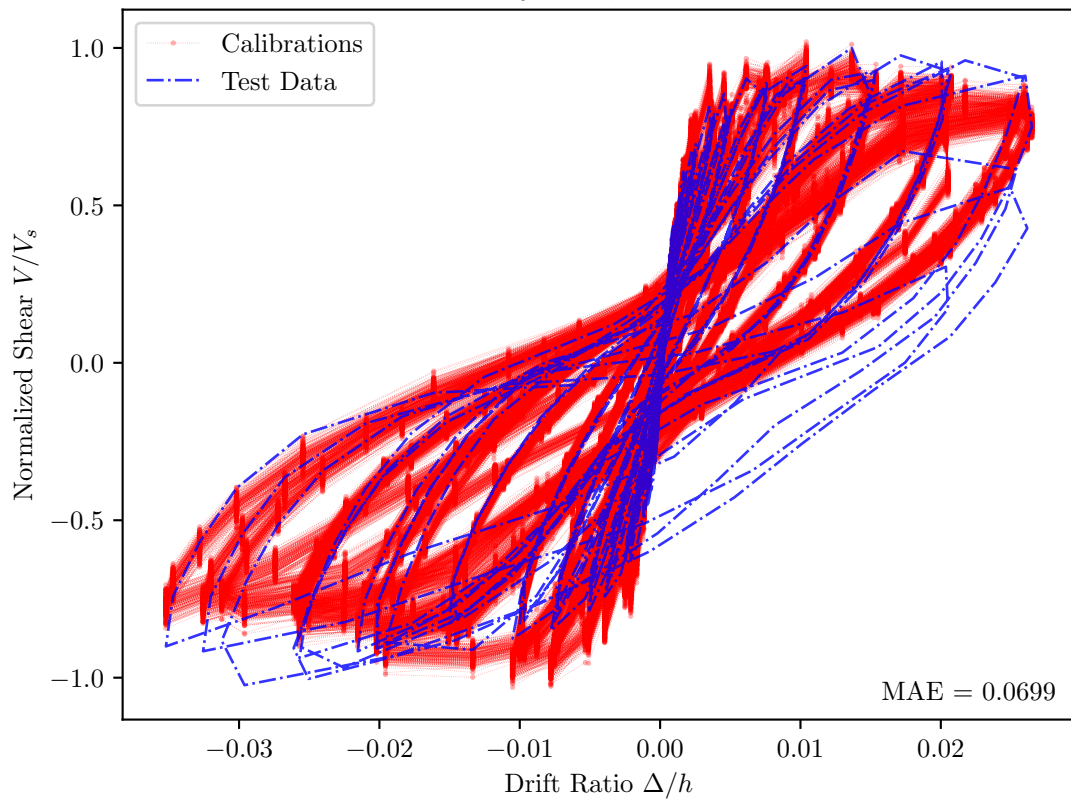
Benzoni and Priestley 1994, NR1 — PEER Id = 357
