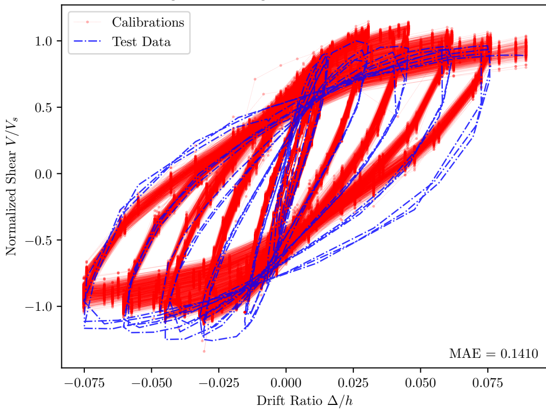
Saatcioglu and Baingo 1999, RC1 — PEER Id = 380
