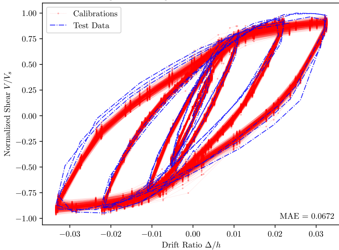
Saatcioglu and Baingo 1999, RC4 — PEER Id = 383
