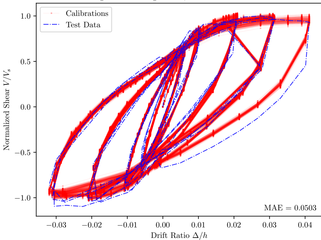
Saatcioglu and Baingo 1999, RC6 — PEER Id = 384
