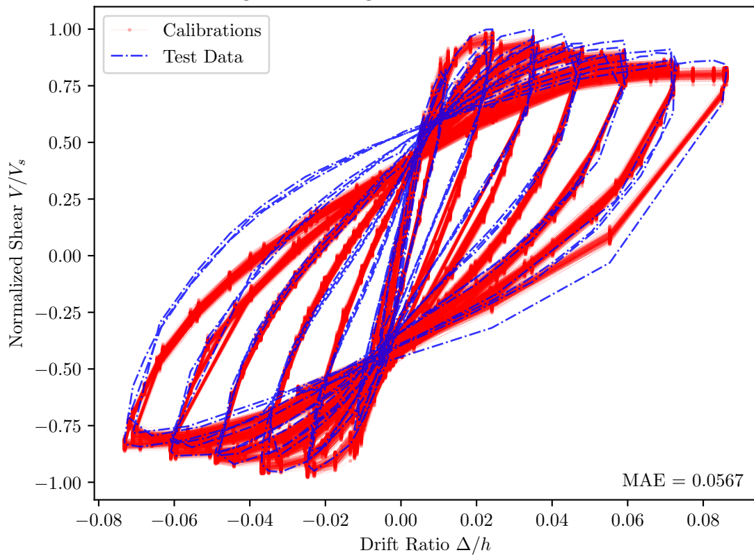
Saatcioglu and Baingo 1999, RC7 — PEER Id = 385
