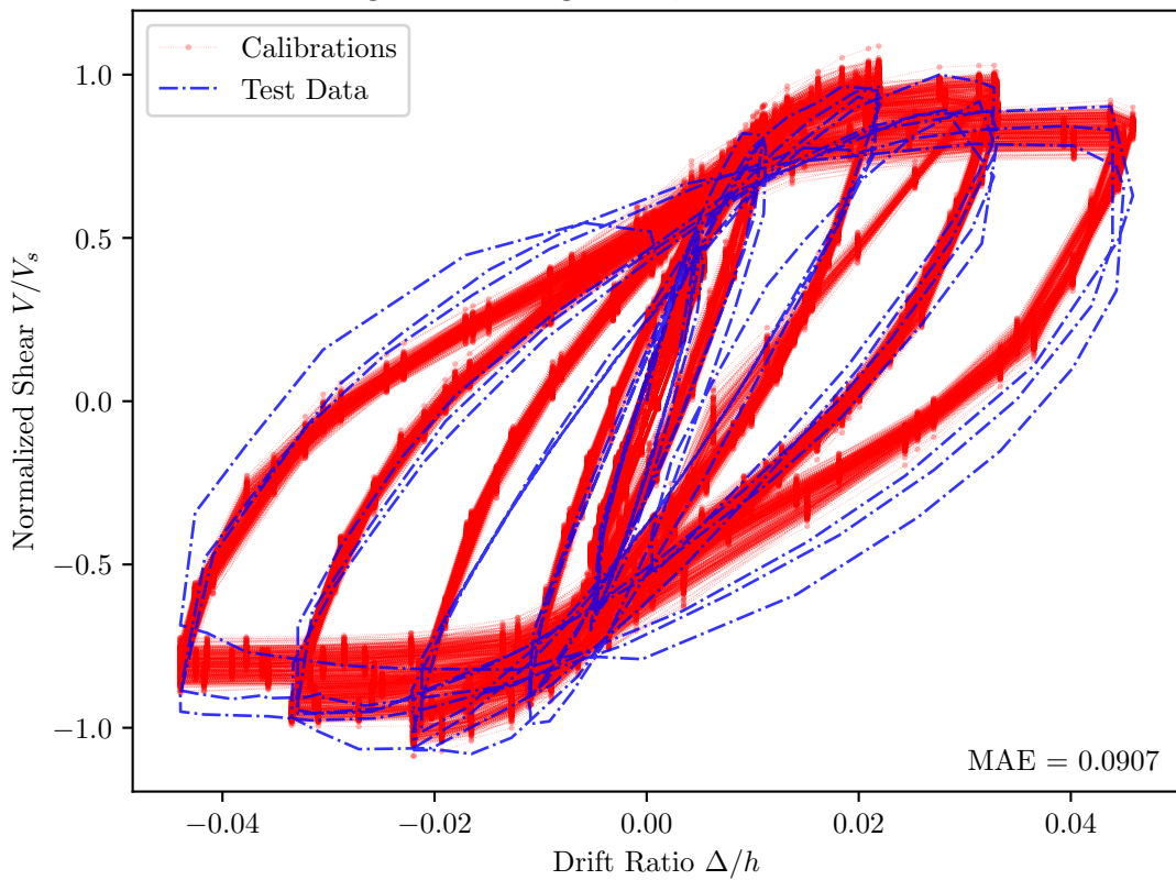
Saatcioglu and Baingo 1999, RC8 — PEER Id = 386
