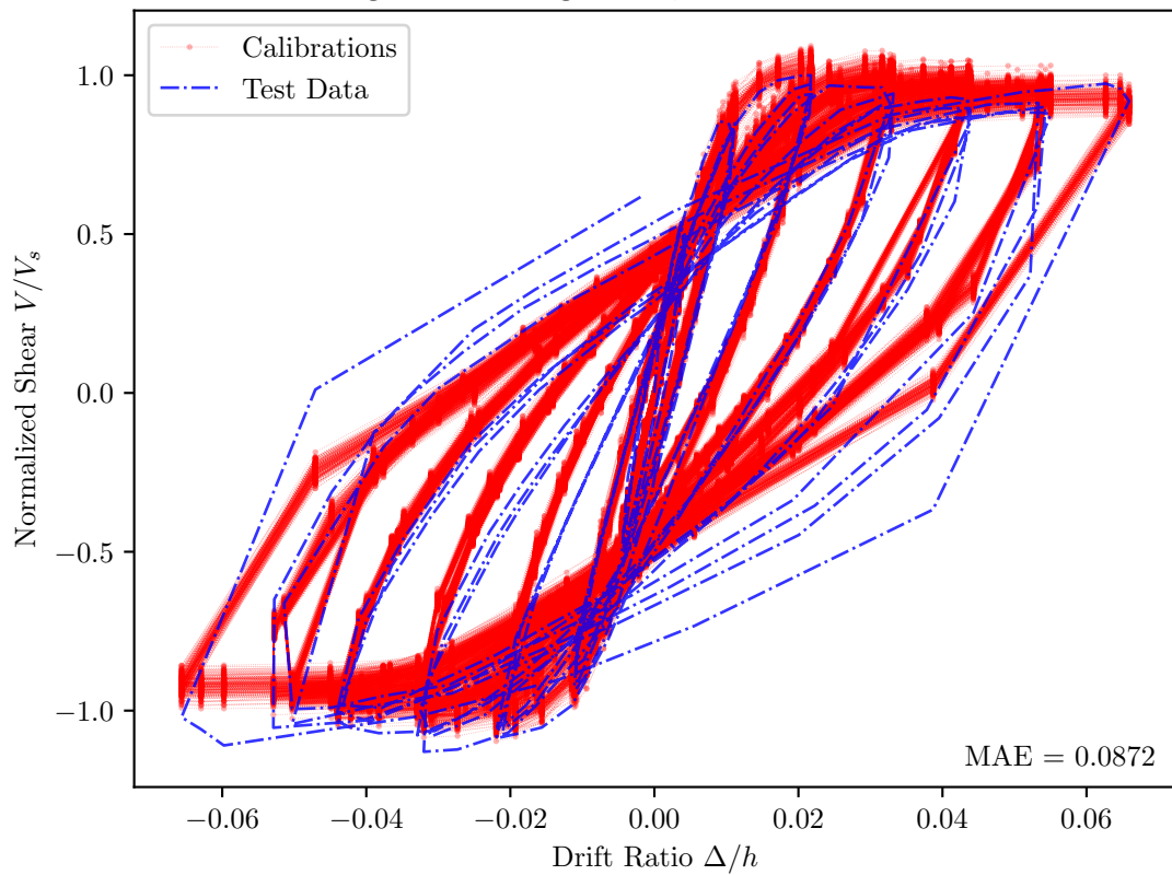
Saatcioglu and Baingo 1999, RC9 — PEER Id = 387
