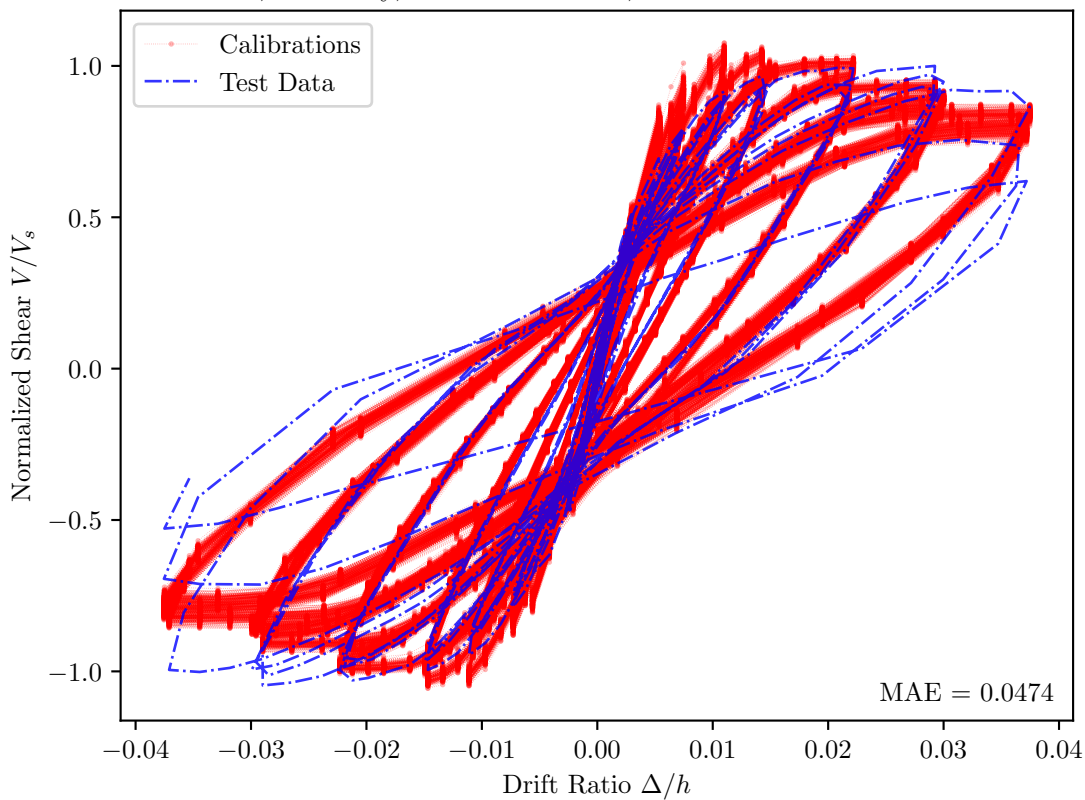
Chai, Priestley, and Seible 1991, Test 3 — PEER Id = 394
