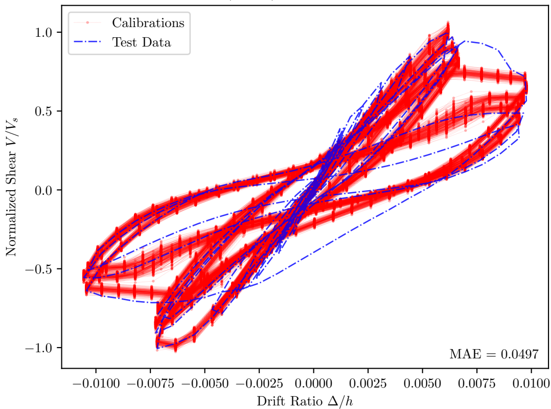
McDaniel, 1997, S1-2 — PEER Id = 415
