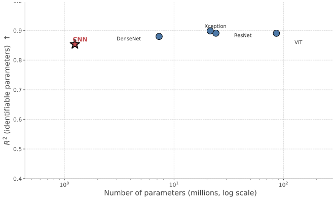
Figure 12: Mean R^2 over the identifiable Hamiltonian parameters as a function of the number of trainable weights (log scale) for the five evaluated architectures. The nearly flat trend—with the compact conventional CNN already matching the accuracy of models two orders of magnitude larger—indicates that predictive accuracy is limited by the physical information available in the s_z projection rather than by model capacity.
