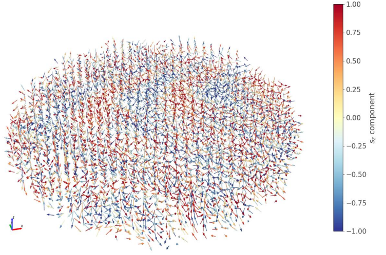
(b) 3D spin configuration — all layers
