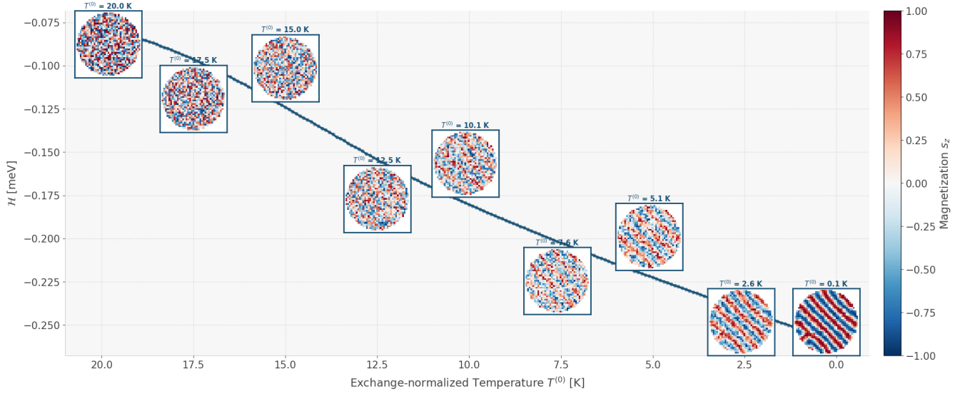
Figure 9: Thermodynamic convergence of a representative magnetic nanodot during simulated annealing. The main panel shows the total Hamiltonian energy \mathcal{H} [meV] as a function of the exchange-normalized annealing temperature T^{(0)} [K] under the fixed parameter configuration. Each inset depicts the two-dimensional out-of-plane magnetization field s_z of the central layer at the corresponding thermal state, illustrating the progressive transition from a fully disordered paramagnetic phase at high T^{(0)} to a thermodynamically relaxed labyrinthine domain configuration at T^{(0)} = 0.1 K, driven by the competing energetic contributions of \tilde{J}_1 and \tilde{K}_{DM} .
