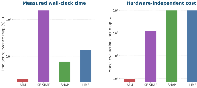
Figure 25: Computational cost of the interpretability methods. Left: measured wall-clock time per relevance map (log scale). Right: hardware-independent cost as the number of model evaluations per map (log scale). A RAM requires a single backward pass (one model evaluation), against \sim 10^3 evaluations for LIME and SHAP and 128 for SF-SHAP, yielding an efficiency advantage of one to two orders of magnitude.
