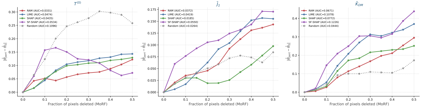
Figure 23: Deletion curves (Most Relevant First) for RAM, LIME, SHAP, and SF-SHAP, with a random-relevance lower bound, for the three representative parameters T^{(0)} , \tilde{J}_2 , and \tilde{K}_{DM} . The vertical axis is the induced deviation |\hat{\theta}_{\text{pert}} - \hat{\theta}_0| as the most relevant pixels are progressively replaced by the baseline; the area under each curve (AUC, reported in the legend) quantifies faithfulness. For the spatially localized \tilde{K}_{DM} all attribution methods lie well above the random baseline, whereas for the global parameter T^{(0)} no method separates from random, reflecting its delocalized thermodynamic nature.
