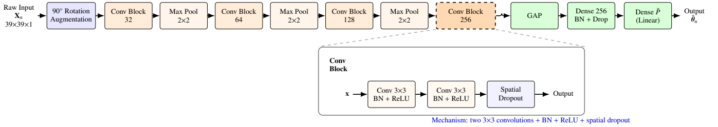
Figure 2: Conventional CNN baseline pipeline for Hamiltonian parameter estimation. The native-resolution single-channel s_z map is augmented on the fly with 90° rotations and processed by four convolutional stages of increasing width interleaved with spatial max-pooling. A detailed view illustrates the internal structure of each convolutional block, composed of two 3×3 convolutions with batch normalization, ReLU activation, and spatial dropout. The final feature maps are aggregated via Global Average Pooling (GAP) and mapped to the physical constants through the customized regression head.
