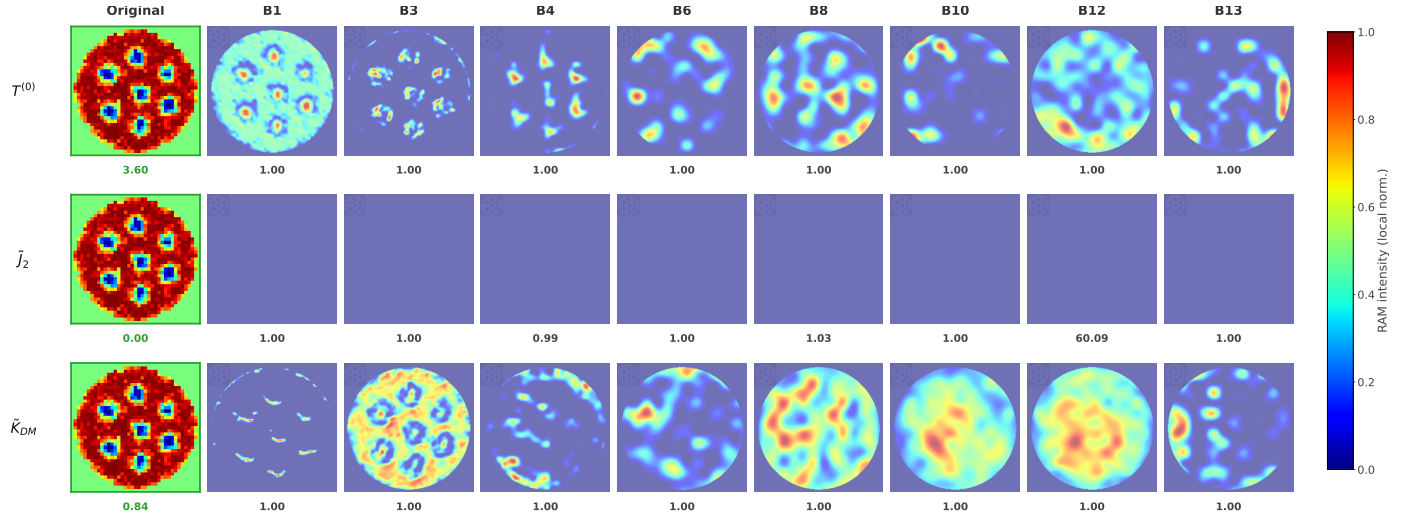
Figure 20: RAMs \tilde{\mathcal{R}}_{\text{RAM}}^{(l,p)} for the Xception architecture, shown for the skyrmion phase, selected as the most representative case from the five-phase RAM computation. Three Hamiltonian parameters \{T^{(0)}, \tilde{J}_2, \tilde{K}_{DM}\} are shown (rows). Each panel displays the RAM overlay (jet colormap) on the original s_z magnetization image (leftmost column), with local per-cell normalization to reveal spatial attribution patterns at each layer independently. Columns correspond to network layers from block1 (entry, 112 \times 112 ) to block13 (exit, 14 \times 14 ). The numerical score below each RAM cell reports the fraction of activation concentrated within the nanodot disk boundary, and the value below each original image reports the ground-truth parameter value for that representative sample. The \tilde{K}_{DM} activations localize on the skyrmion cores, while \tilde{J}_2 remains inactive (vanishing value in this phase), illustrating a physically consistent hierarchical decoupling: early layers capture the chiral core structure while deeper layers consolidate activations into topologically significant spatial hotspots.
