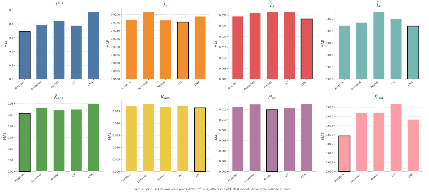
Figure 14: Per-variable Mean Absolute Error (MAE) across the five evaluated architectures for the eight Hamiltonian parameters \theta , reported on the held-out test set in the original physical units of each parameter (K for T^{(0)} , meV for exchange and DMI constants, and meV/atom for anisotropy and external field parameters). Each panel corresponds to one target parameter and shows one bar per architecture. The comparatively larger MAE observed for T^{(0)} , \tilde{J}_2 , and \tilde{K}_{DM} — reaching up to 0.49 K, 0.021 meV, and 0.037 meV respectively in the worst-performing architecture — is attributable to the thermally disordered paramagnetic configurations populating the high-temperature regime of the dataset (see Figure 11), where configurations generated by widely different parameter values relax into statistically similar noise textures, inflating the absolute error even when the global R^2 correlation remains strong. The comparatively small MAE of \tilde{J}_3 and \tilde{J}_4 despite their near-zero R^2 reflects the narrow dynamic range of these parameters in the dataset rather than genuine predictive skill. Black-bordered bars indicate the best-performing architecture for each parameter.
