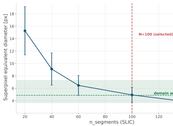
Figure 22: Physical criterion for the SLIC segmentation used by the perturbation-based baselines. The superpixel equivalent diameter is plotted against the number of SLIC segments; the selected value N = 100 (dashed red) yields superpixels whose size matches the characteristic magnetic domain width ( \approx 4.9 px, dashed green), so that each interpretable region corresponds to a single magnetic domain.
