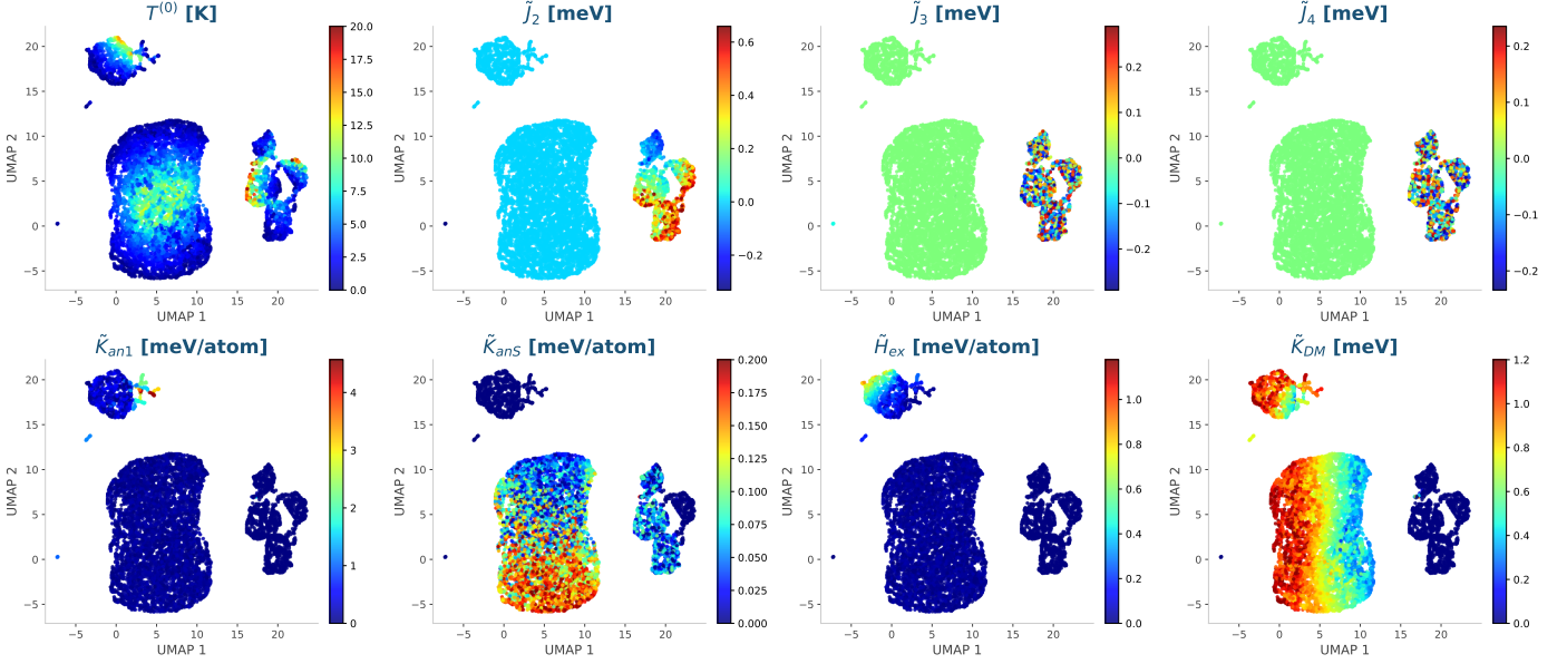
Figure 15: UMAP-based 2D projection of the Xception latent space on the held-out test set, colored by each of the eight Hamiltonian parameters \theta = [T^{(0)}, \tilde{J}_2, \tilde{J}_3, \tilde{J}_4, \tilde{K}_{an1}, \tilde{K}_{anS}, \tilde{H}_{ex}, \tilde{K}_{DM}] . Each point represents a magnetization image \mathbf{X}_n projected from the high-dimensional feature space of the Xception backbone into two dimensions via UMAP.
