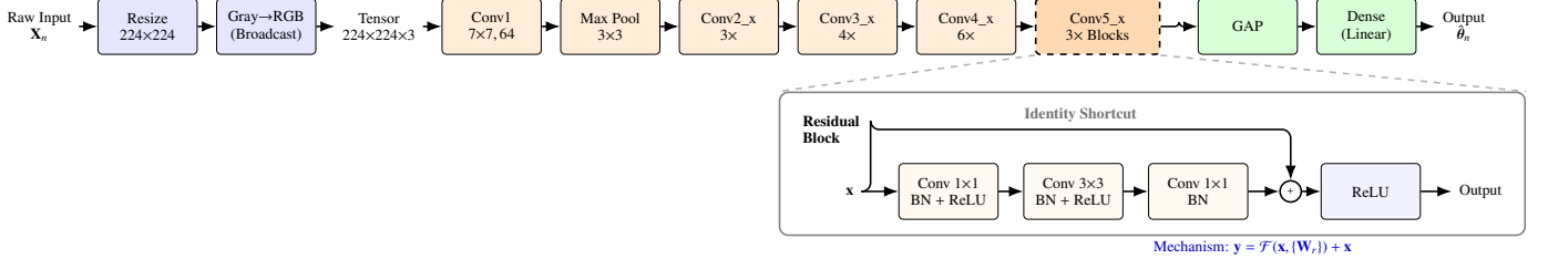
Figure 3: ResNet50 architecture pipeline for Hamiltonian parameter estimation. The pipeline progresses from single-channel input preprocessing through a feature extractor trained from scratch. The Residual bottleneck structure used extensively in Conv5_x. The deepest features are processed by the customized regression head containing a Global Average Pooling (GAP) and a final dense layer with linear activation to output the predicted physical constants.
