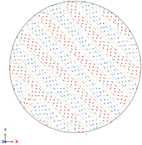
(a) 2D spin configuration — central layer z = 3
