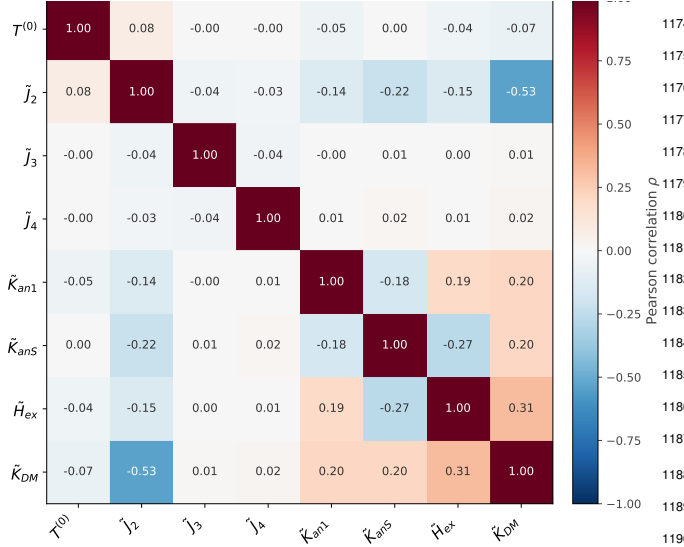
Figure 8: Pairwise Pearson correlation matrix of the eight Hamiltonian parameters computed over the entire dataset of 166,141 configurations. All parameter pairs are essentially uncorrelated ( |\rho| \lesssim 0.3 ), with the single exception of the second-shell exchange \tilde{J}_2 and the DMI strength \tilde{K}_{DM} ( \rho \approx -0.53 ), whose anti-correlation is a direct consequence of the deliberate design in which the exchange-frustration and chiral mechanisms are activated in a mutually exclusive fashion. The absence of spurious cross-parameter correlations indicates that the model cannot exploit artificial statistical shortcuts to infer one parameter from another.
