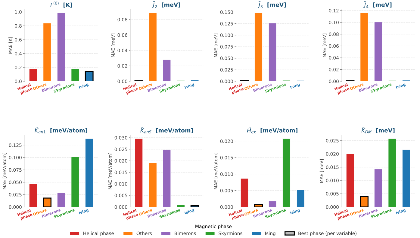
Figure 18: Per-phase Mean Absolute Error (MAE) of the best-performing model, Xception, across all eight Hamiltonian parameters \theta for the five identified magnetic phase categories, reported in the original physical units of each parameter after inverse Min-Max scaling. Each panel corresponds to one target parameter and shows one bar per magnetic phase. The others and bimeron categories consistently concentrate the largest absolute errors across most parameters, confirming that the thermally disordered, transitional, and mixed-chirality configurations within these groups constitute the primary source of prediction error in the global regression analysis. Black-bordered bars indicate the magnetic phase with the lowest MAE for each parameter.
