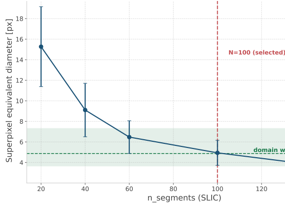
Figure 11: Physical criterion for the SLIC segmentation used by the perturbation-based baselines. The superpixel equivalent diameter is plotted against the number of SLIC segments; the selected value N = 100 (dashed red) yields superpixels whose size matches the characteristic magnetic domain width ( \approx 4.9 px, dashed green), so that each interpretable region corresponds to a single magnetic domain.
