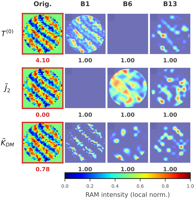
Figure 9: RAMs \tilde{K}_{\text{RAM}}^{(l,p)} for the Xception architecture in the helical phase. Rows are three Hamiltonian parameters \{T^{(0)}, \tilde{J}_2, \tilde{K}_{DM}\} ; columns are three representative network layers, block1 (entry, B1), block6 (middle, B6), and block13 (exit, B13), with the original s_z image in the leftmost column. Each panel overlays the RAM intensity (locally normalized) on the magnetization; the value below each original image is the ground-truth parameter.
