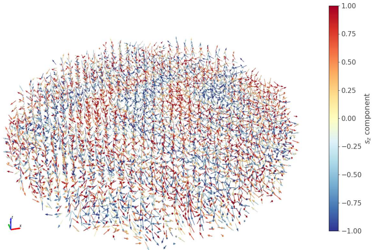
(b) 3D spin configuration — all layers
