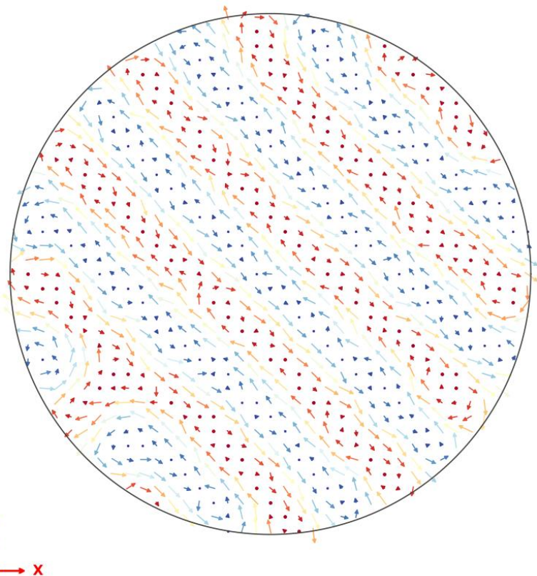
(a) 2D spin configuration — central layer z = 3
