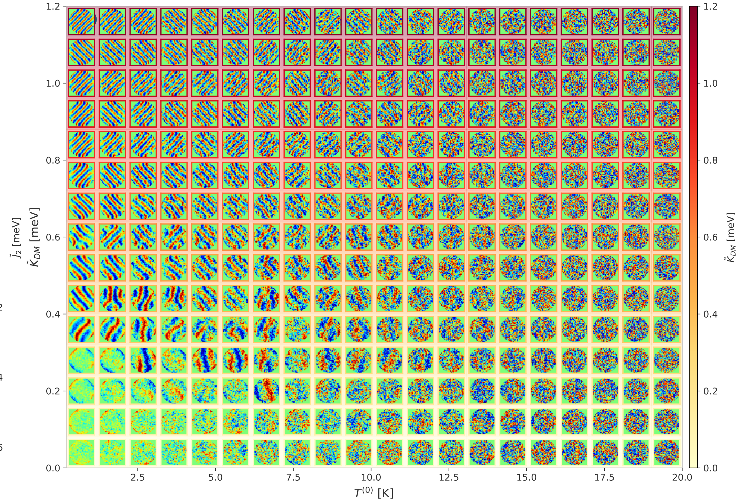
Dataset Phase Space — Representative Magnetization Images
