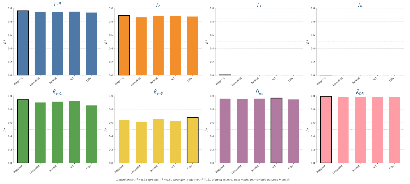
Figure 14: Per-variable R^2 score across the five evaluated architectures (Xception, DenseNet, ResNet, ViT, and the conventional CNN baseline) for the eight Hamiltonian parameters \theta , reported on the held-out test set. Each panel corresponds to one target parameter and shows one bar per architecture. Negative R^2 values, indicating predictions no better than the dataset mean, are clipped to zero for visualization clarity. Black-bordered bars indicate the best-performing architecture for each parameter.
