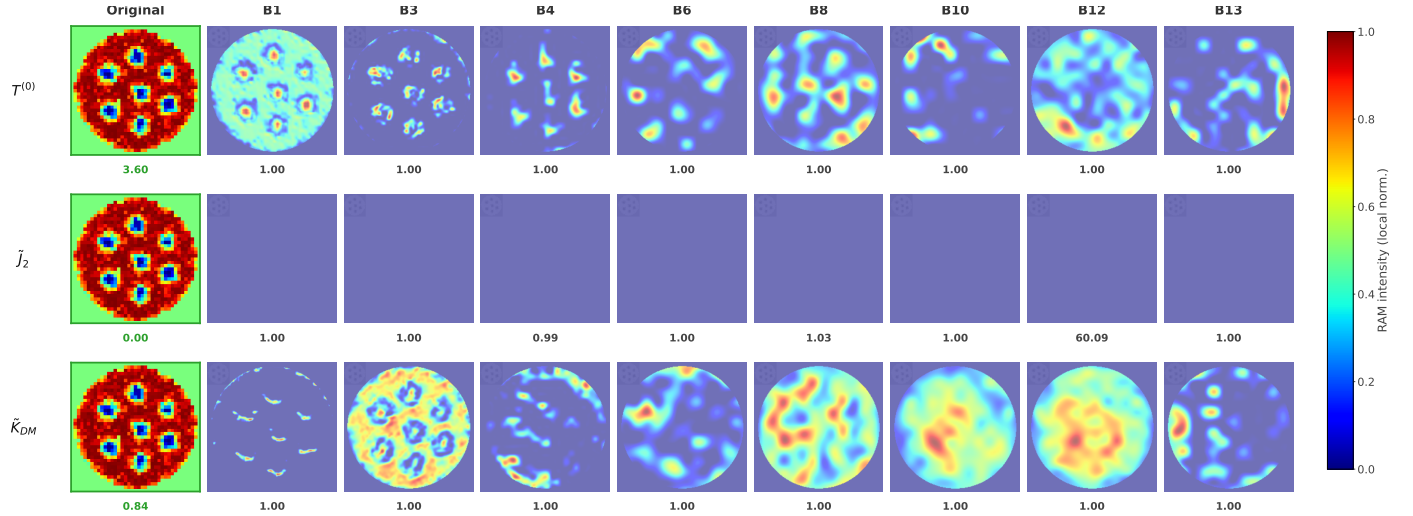
Figure 21: RAMs \tilde{R}_{\text{RAM}}^{(l,p)} for the Xception architecture, shown for the skyrmion phase, selected as the most representative case from the five-phase RAM computation. Three Hamiltonian parameters \{T^{(0)}, \tilde{J}_2, \tilde{K}_{DM}\} are shown (rows). Each panel displays the RAM overlay (jet colormap) on the original s_z magnetization image (leftmost column), with local per-cell normalization to reveal spatial attribution patterns at each layer independently. Columns correspond to network layers from block1 (entry, 112 \times 112 ) to block13 (exit, 14 \times 14 ). The numerical score below each RAM cell reports the fraction of activation concentrated within the nanodot disk boundary, and the value below each original image reports the ground-truth parameter value for that representative sample. The \tilde{K}_{DM} activations localize on the skyrmion cores, while \tilde{J}_2 remains inactive (vanishing value in this phase), illustrating a physically consistent hierarchical decoupling: early layers capture the chiral core structure while deeper layers consolidate activations into topologically significant spatial hotspots.
