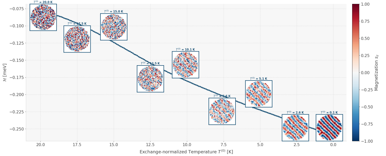
Figure 10: Thermodynamic convergence of a representative magnetic nanodot during simulated annealing. The main panel shows the total Hamiltonian energy \mathcal{H} [meV] as a function of the exchange-normalized annealing temperature T^{(0)} [K] under the fixed parameter configuration. Each inset depicts the two-dimensional out-of-plane magnetization field s_z of the central layer at the corresponding thermal state, illustrating the progressive transition from a fully disordered paramagnetic phase at high T^{(0)} to a thermodynamically relaxed labyrinthine domain configuration at T^{(0)} = 0.1 K, driven by the competing energetic contributions of \tilde{J}_1 and \tilde{K}_{DM} .
