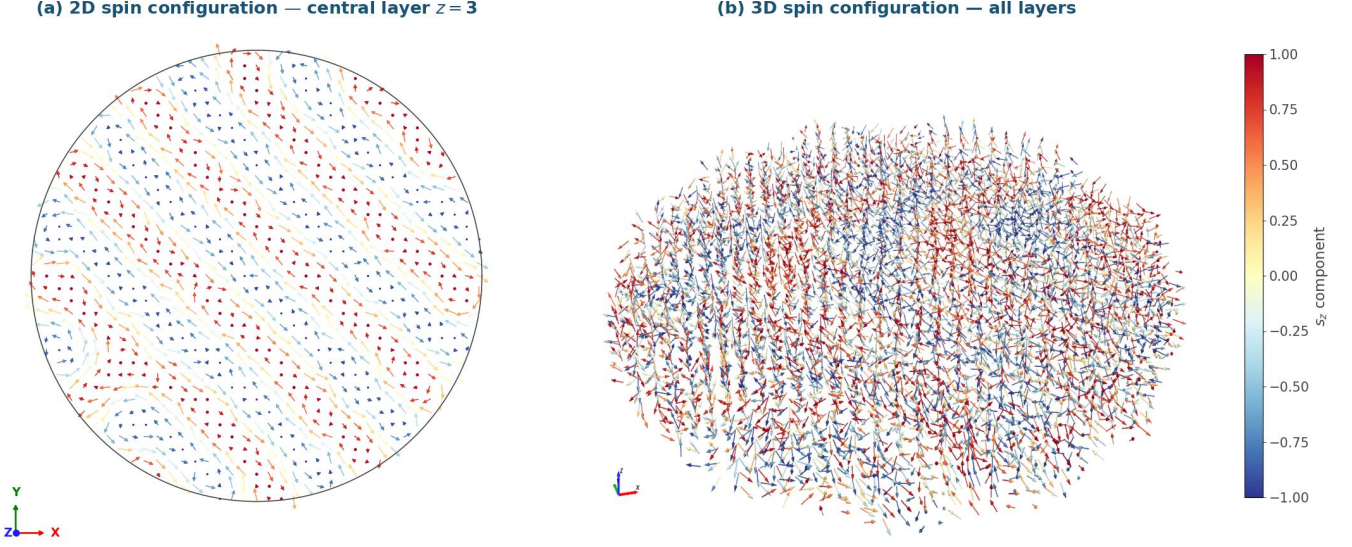
Figure 11: Converged ground-state spin configuration of a representative magnetic nanodot at T_{final}^{(0)} = 0.1 K under a fixed parameter configuration. (a) Two-dimensional projection of the out-of-plane magnetization field s_z : colored dots indicate spins oriented predominantly out-of-plane, while colored arrows represent the in-plane orientation ( s_x, s_y ) of transverse moments. (b) Full three-dimensional spin configuration, revealing the volumetric coherence of the labyrinthine chiral domain structure stabilized by the competition between \tilde{J}_1 and \tilde{K}_{DM} . Color encodes the s_z component.
