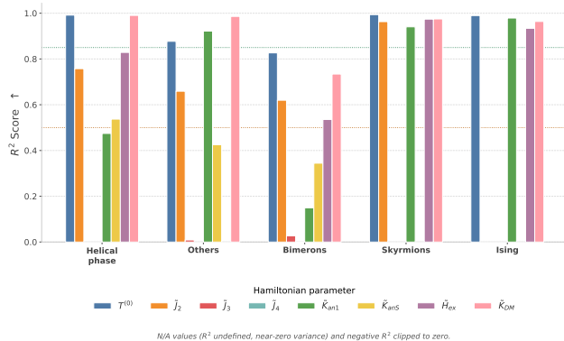
Figure 18: Per-phase R^2 score of the best-performing model, Xception, across all eight Hamiltonian parameters \theta for the five identified magnetic phase categories. Each bar group corresponds to one magnetic phase and each bar to one target parameter. Dashed horizontal lines mark the identifiability thresholds at R^2 = 0.85 (high predictability) and R^2 = 0.50 (partial predictability). Negative R^2 values and near-zero variance cases (N/A) are clipped to zero. The Skyrmion and Ising phases achieve near-perfect accuracy across the identifiable parameters, while the Bimeron and Others phases exhibit the lowest identifiability owing to their weakly discriminative, structurally ambiguous magnetization textures.
