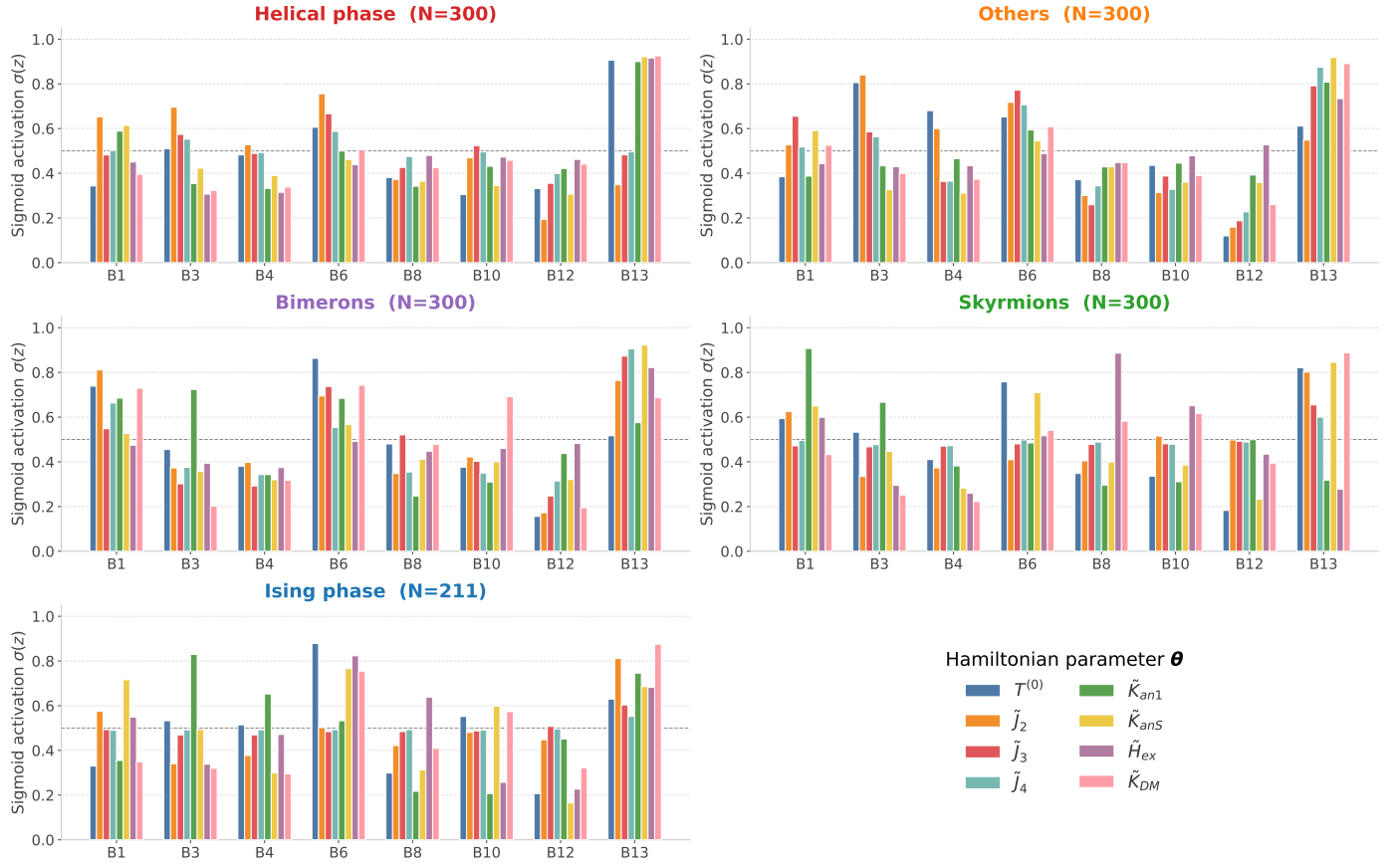
Figure 22: Mean maximum RAM activation per network layer and Hamiltonian parameter \theta , averaged over N = 300 test samples per magnetic phase ( N = 211 for the Ising phase; Xception CNN). Activations are reported after sigmoid normalization \sigma\left(\frac{x-\mu}{\sigma_x}\right) applied globally per variable, where values above \sigma = 0.5 indicate above-average gradient response. Each color corresponds to a distinct parameter following the nomenclature of Table 2. Activation is measured exclusively within the nanodot disk boundary (masked RAM). The depth profile peaks at the terminal exit-flow layer block13, where the network aggregates the global representations of the identifiable parameters, with secondary peaks in the middle-flow layers where localized chiral and domain-wall features are assembled. The higher-order exchange constants \tilde{J}_3 and \tilde{J}_4 consistently exhibit the lowest sigmoid activation across all layers and phases, confirming the fundamental identifiability limit identified in the regression analysis.
