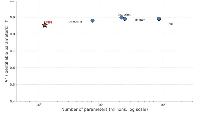
Figure 13: Mean R^2 over the identifiable Hamiltonian parameters as a function of the number of trainable weights (log scale) for the five evaluated architectures. The nearly flat trend—with the compact conventional CNN already matching the accuracy of models two orders of magnitude larger—indicates that predictive accuracy is limited by the physical information available in the s_z projection rather than by model capacity.
