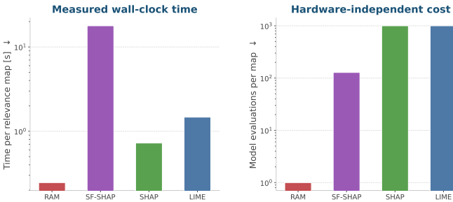
Figure 26: Computational cost of the interpretability methods. Left: measured wall-clock time per relevance map (log scale). Right: hardware-independent cost as the number of model evaluations per map (log scale). A RAM requires a single backward pass (one model evaluation), against \sim 10^3 evaluations for LIME and SHAP and 128 for SF-SHAP, yielding an efficiency advantage of one to two orders of magnitude.
