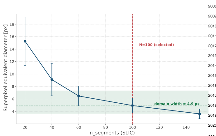
Figure 23: Physical criterion for the SLIC segmentation used by the perturbation-based baselines. The superpixel equivalent diameter is plotted against the number of SLIC segments; the selected value N = 100 (dashed red) yields superpixels whose size matches the characteristic magnetic domain width ( \approx 4.9 px, dashed green), so that each interpretable region corresponds to a single magnetic domain.
