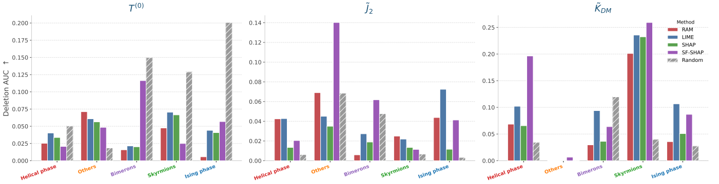
Figure 25: Deletion AUC resolved by magnetic phase for RAM, LIME, SHAP, and SF-SHAP (with the random baseline), for T^{(0)} , \tilde{J}_2 , and \tilde{K}_{DM} . RAMs attain a faithfulness comparable to the perturbation-based methods and far above the random baseline for the localized \tilde{K}_{DM} , especially in the ordered skyrmion and Ising phases, whereas the delocalized T^{(0)} shows no method separating from random.
