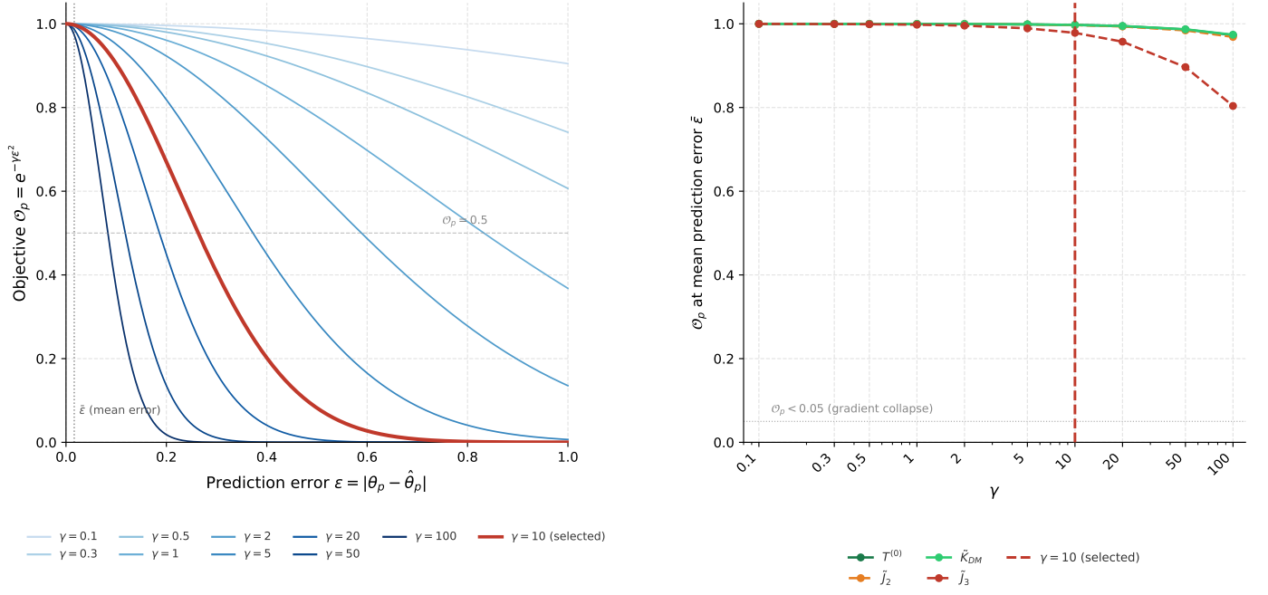
Figure 20: Sensitivity analysis of the RAM precision factor \gamma . Left: shape of the Gaussian objective O_p = e^{-\gamma \epsilon^2} as a function of the prediction error \epsilon = |\theta_p - \hat{\theta}_p| for \gamma \in \{0.1, \dots, 100\} ; the selected value \gamma = 10 is highlighted in red. The vertical dotted line indicates the empirical mean error \bar{\epsilon} on the test set. Right: O_p evaluated at \bar{\epsilon} for each Hamiltonian parameter as a function of \gamma . The horizontal dotted line marks the gradient collapse threshold O_p = 0.05 . The identifiable parameters ( T^{(0)} , J_2 , \tilde{K}_{DM} ) remain near O_p \approx 1 across the full \gamma range owing to their small mean errors; only the poorly identified \tilde{J}_3 declines at high \gamma , and even then stays well above the collapse threshold. The value \gamma = 10 is selected as a selective yet well-conditioned operating point.
