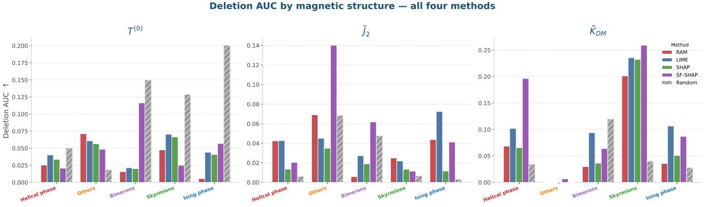
Figure 25: Deletion AUC resolved by magnetic phase for RAM, LIME, SHAP, and SF-SHAP (with the random baseline), for T^{(0)} , \tilde{J}_2 , and \tilde{K}_{DM} . RAMs attain a faithfulness comparable to the perturbation-based methods and far above the random baseline for the localized \tilde{K}_{DM} , especially in the ordered skyrmion and Ising phases, whereas the delocalized T^{(0)} shows no method separating from random.
