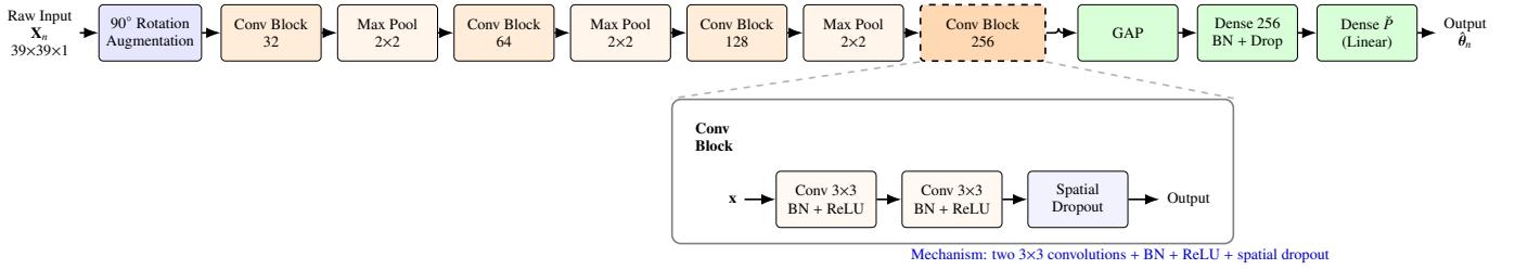
Figure 2: Conventional CNN baseline pipeline for Hamiltonian parameter estimation. The native-resolution single-channel s_z map is augmented on the fly with 90^\circ rotations and processed by four convolutional stages of increasing width interleaved with spatial max-pooling. A detailed view illustrates the internal structure of each convolutional block, composed of two 3 \times 3 convolutions with batch normalization, ReLU activation, and spatial dropout. The final feature maps are aggregated via Global Average Pooling (GAP) and mapped to the physical constants through the customized regression head.
