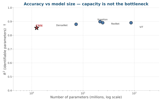
Figure 13: Mean R^2 over the identifiable Hamiltonian parameters as a function of the number of trainable weights (log scale) for the five evaluated architectures. The nearly flat trend—with the compact conventional CNN already matching the accuracy of models two orders of magnitude larger—indicates that predictive accuracy is limited by the physical information available in the s_z projection rather than by model capacity.
