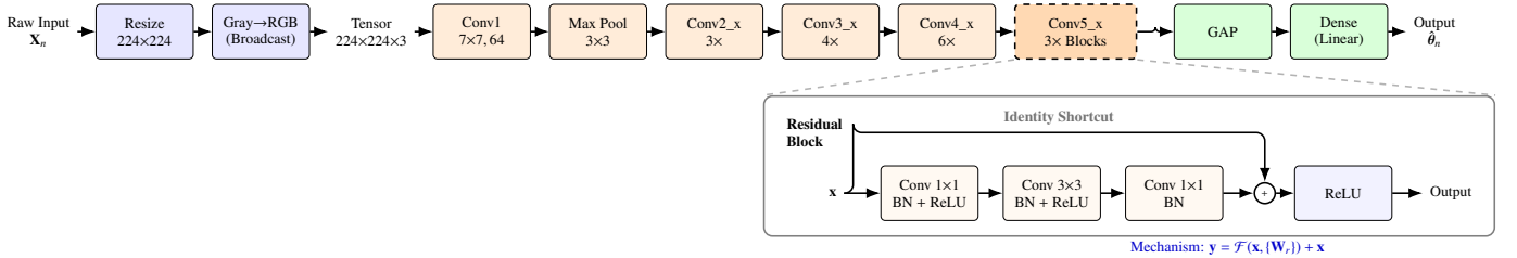
Figure 3: ResNet50 architecture pipeline for Hamiltonian parameter estimation. The pipeline progresses from single-channel input preprocessing through a feature extractor trained from scratch. The Residual bottleneck structure used extensively in Conv5_x. The deepest features are processed by the customized regression head containing a Global Average Pooling (GAP) and a final dense layer with linear activation to output the predicted physical constants.
