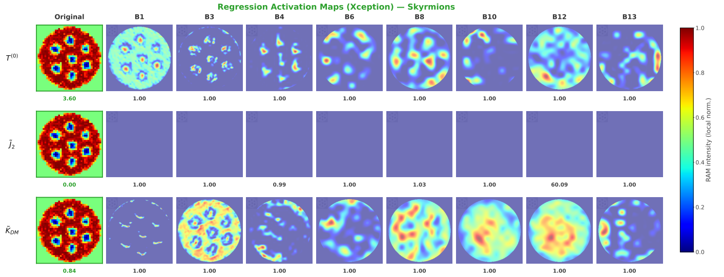
Figure 21: RAMs \tilde{\mathcal{R}}_{\text{RAM}}^{(l,p)} for the Xception architecture, shown for the skyrmion phase, selected as the most representative case from the five-phase RAM computation. Three Hamiltonian parameters \{T^{(0)}, \tilde{J}_2, \tilde{K}_{DM}\} are shown (rows). Each panel displays the RAM overlay (jet colormap) on the original s_z magnetization image (leftmost column), with local per-cell normalization to reveal spatial attribution patterns at each layer independently. Columns correspond to network layers from block1 (entry, 112 \times 112 ) to block13 (exit, 14 \times 14 ). The numerical score below each RAM cell reports the fraction of activation concentrated within the nanodisk boundary, and the value below each original image reports the ground-truth parameter value for that representative sample. The \tilde{K}_{DM} activations localize on the skyrmion cores, while \tilde{J}_2 remains inactive (vanishing value in this phase), illustrating a physically consistent hierarchical decoupling: early layers capture the chiral core structure while deeper layers consolidate activations into topologically significant spatial hotspots.
