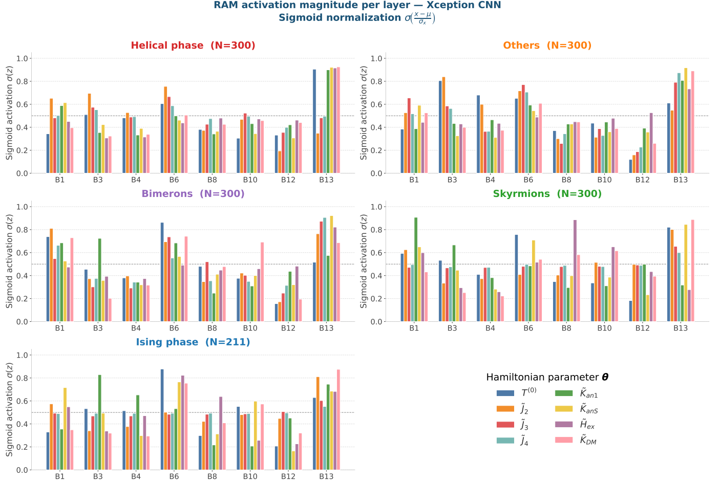
Figure 22: Mean maximum RAM activation per network layer and Hamiltonian parameter \theta , averaged over N = 300 test samples per magnetic phase ( N = 211 for the Ising phase; Xception CNN). Activations are reported after sigmoid normalization \sigma\left(\frac{x-\mu}{\sigma_x}\right) applied globally per variable, where values above \sigma = 0.5 indicate above-average gradient response. Each color corresponds to a distinct parameter following the nomenclature of Table 2. Activation is measured exclusively within the nanodot disk boundary (masked RAM). The depth profile peaks at the terminal exit-flow layer block13, where the network aggregates the global representations of the identifiable parameters, with secondary peaks in the middle-flow layers where localized chiral and domain-wall features are assembled. The higher-order exchange constants \tilde{J}_3 and \tilde{J}_4 consistently exhibit the lowest sigmoid activation across all layers and phases, confirming the fundamental identifiability limit identified in the regression analysis.
