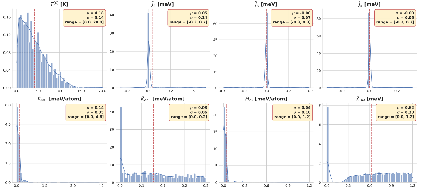
Figure 9: Empirical distributions of the thermodynamic and Hamiltonian parameters \{T^{(0)}, \tilde{J}_2, \tilde{J}_3, \tilde{J}_4, \tilde{K}_{an1}, \tilde{K}_{an5}, \tilde{H}_{ex}, \tilde{K}_{DM}\} used to generate the dataset. Each subplot presents a histogram and KDE for a given variable, along with summary statistics including mean, standard deviation, and value range.
