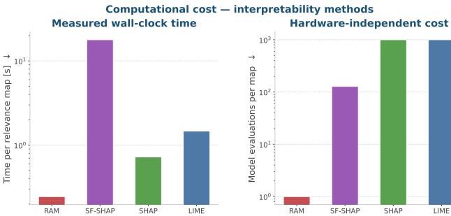
Figure 26: Computational cost of the interpretability methods. Left: measured wall-clock time per relevance map (log scale). Right: hardware-independent cost as the number of model evaluations per map (log scale). A RAM requires a single backward pass (one model evaluation), against \sim 10^3 evaluations for LIME and SHAP and 128 for SF-SHAP, yielding an efficiency advantage of one to two orders of magnitude.
