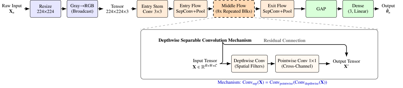
Figure 5: Xception architecture pipeline for Hamiltonian parameter estimation. The feature extractor composed of Entry, Middle, and Exit flows. A detailed horizontal view illustrates the depthwise separable convolution mechanism where spatial feature extraction (depthwise) and cross-channel correlations (pointwise) are entirely decoupled. The final aggregated features are mapped to physical constants.
