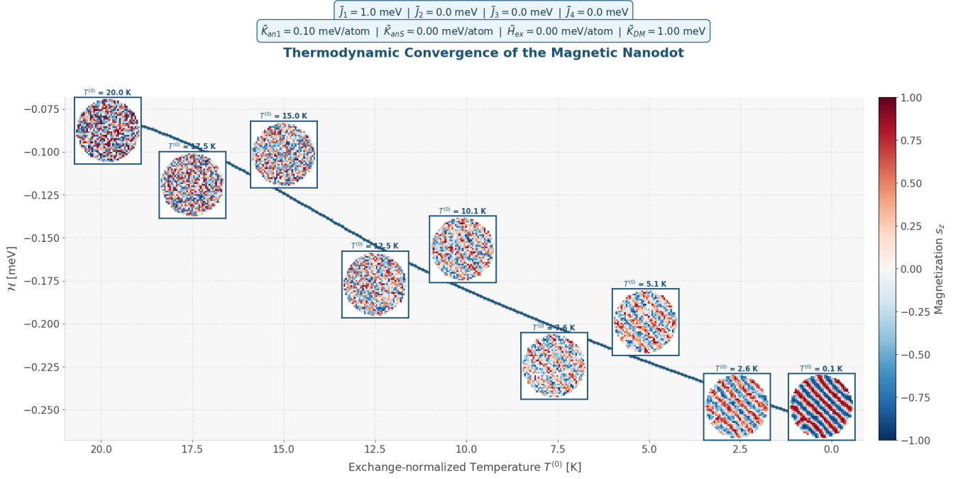
Figure 10: Thermodynamic convergence of a representative magnetic nanodot during simulated annealing. The main panel shows the total Hamiltonian energy \mathcal{H} [meV] as a function of the exchange-normalized annealing temperature T^{(0)} [K] under the fixed parameter configuration. Each inset depicts the two-dimensional out-of-plane magnetization field s_z of the central layer at the corresponding thermal state, illustrating the progressive transition from a fully disordered paramagnetic phase at high T^{(0)} to a thermodynamically relaxed labyrinthine domain configuration at T^{(0)} = 0.1 K, driven by the competing energetic contributions of \tilde{J}_1 and \tilde{K}_{DM} .
