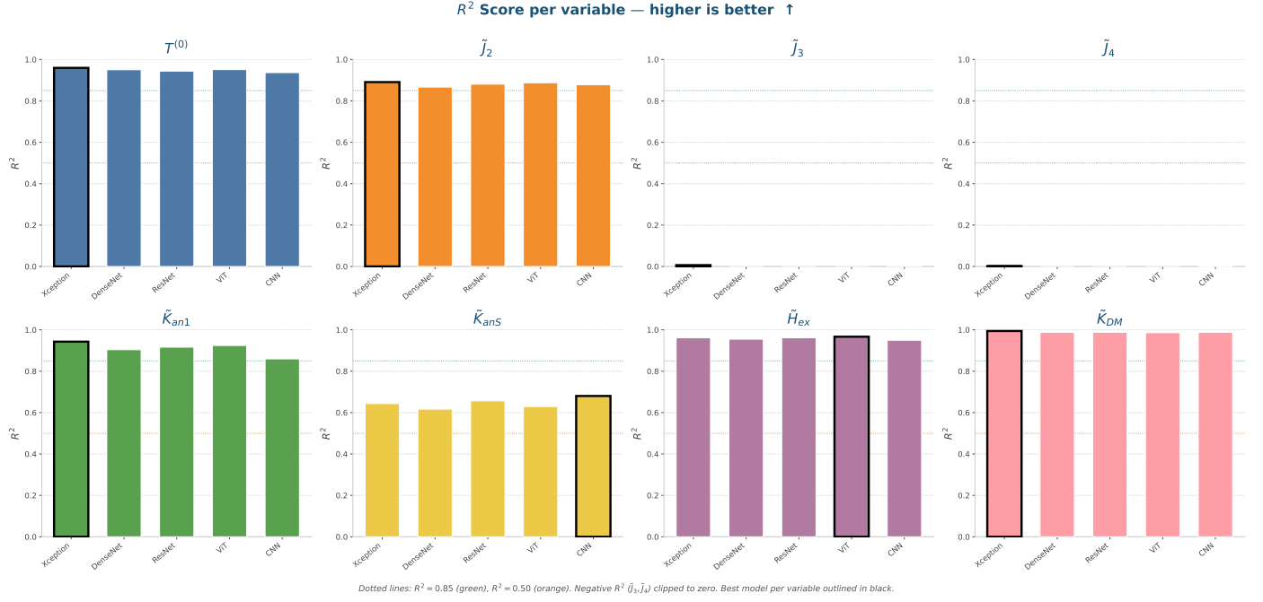
Figure 14: Per-variable R^2 score across the five evaluated architectures (Xception, DenseNet, ResNet, ViT, and the conventional CNN baseline) for the eight Hamiltonian parameters \theta , reported on the held-out test set. Each panel corresponds to one target parameter and shows one bar per architecture. Negative R^2 values, indicating predictions no better than the dataset mean, are clipped to zero for visualization clarity. Black-bordered bars indicate the best-performing architecture for each parameter.
