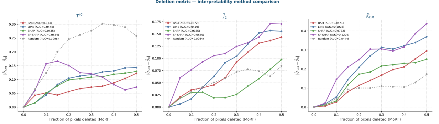
Figure 24: Deletion curves (Most Relevant First) for RAM, LIME, SHAP, and SF-SHAP, with a random-relevance lower bound, for the three representative parameters T^{(0)} , \tilde{J}_2 , and \tilde{K}_{DM} . The vertical axis is the induced deviation |\hat{\theta}_{\text{pert}} - \hat{\theta}_0| as the most relevant pixels are progressively replaced by the baseline; the area under each curve (AUC, reported in the legend) quantifies faithfulness. For the spatially localized \tilde{K}_{DM} all attribution methods lie well above the random baseline, whereas for the global parameter T^{(0)} no method separates from random, reflecting its delocalized thermodynamic nature.
