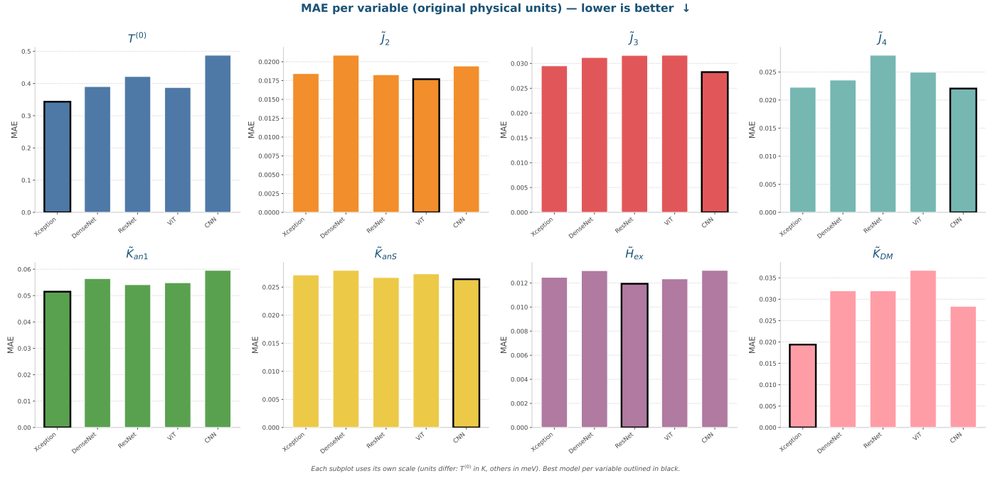
Figure 15: Per-variable Mean Absolute Error (MAE) across the five evaluated architectures for the eight Hamiltonian parameters \theta , reported on the held-out test set in the original physical units of each parameter (K for T^{(0)} , meV for exchange and DMI constants, and meV/atom for anisotropy and external field parameters). Each panel corresponds to one target parameter and shows one bar per architecture. The comparatively larger MAE observed for T^{(0)} , \tilde{J}_2 , and \tilde{K}_{DM} — reaching up to 0.49 K, 0.021 meV, and 0.037 meV respectively in the worst-performing architecture — is attributable to the thermally disordered paramagnetic configurations populating the high-temperature regime of the dataset (see Figure 12), where configurations generated by widely different parameter values relax into statistically similar noise textures, inflating the absolute error even when the global R^2 correlation remains strong. The comparatively small MAE of \tilde{J}_3 and \tilde{J}_4 despite their near-zero R^2 reflects the narrow dynamic range of these parameters in the dataset rather than genuine predictive skill. Black-bordered bars indicate the best-performing architecture for each parameter.
