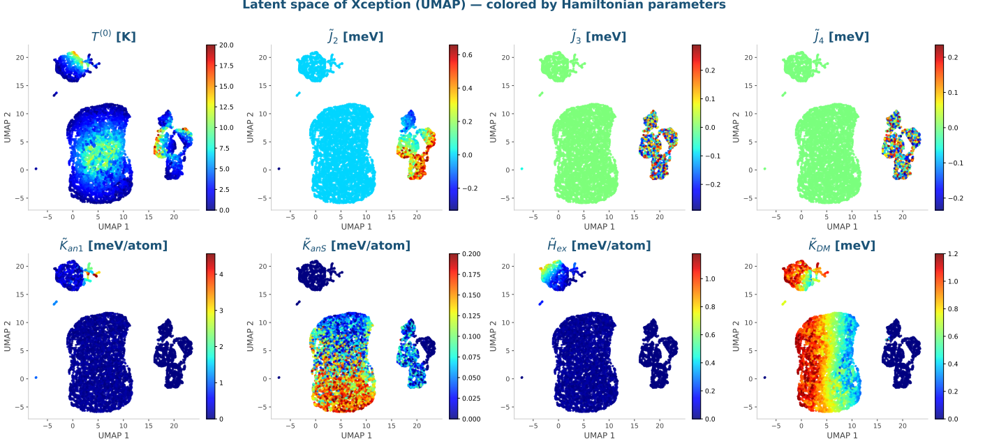
Figure 16: UMAP-based 2D projection of the Xception latent space on the held-out test set, colored by each of the eight Hamiltonian parameters \theta = [T^{(0)}, \tilde{J}_2, \tilde{J}_3, \tilde{J}_4, \tilde{K}_{an1}, \tilde{K}_{anS}, \tilde{H}_{ex}, \tilde{K}_{DM}] . Each point represents a magnetization image \mathbf{X}_n projected from the high-dimensional feature space of the Xception backbone into two dimensions via UMAP.
