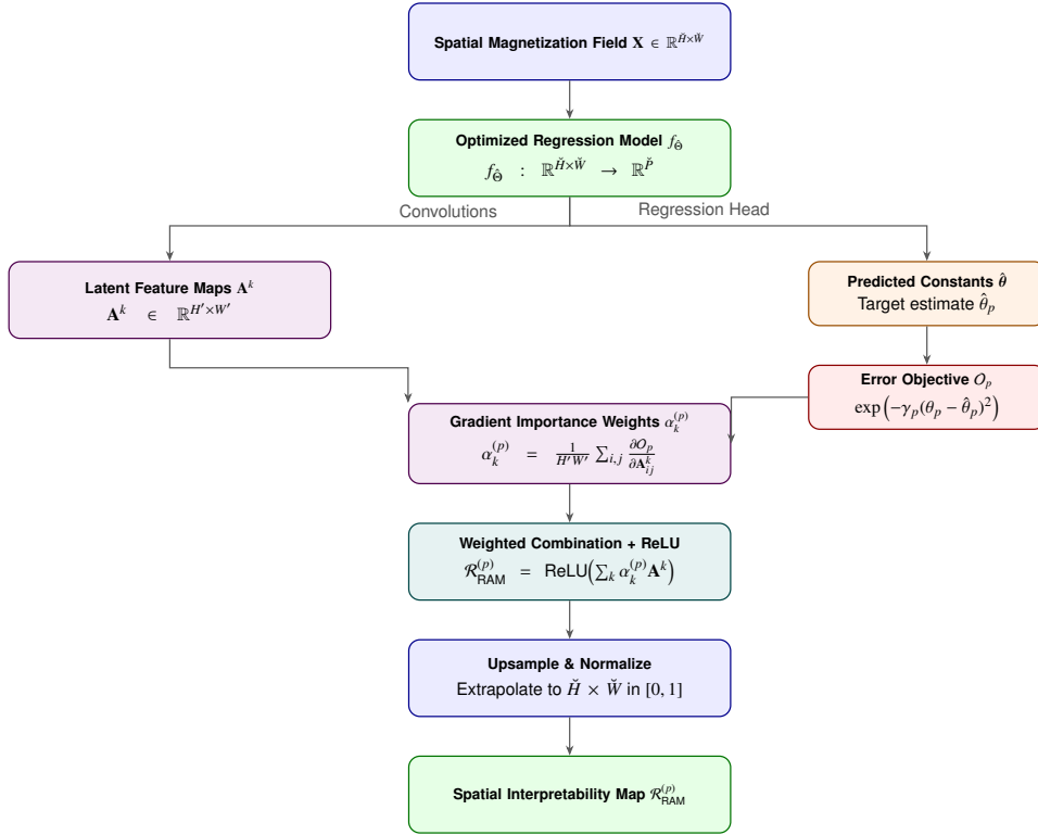
Figure 7: RAMs extraction pipeline. Latent feature maps and continuous predictions from the network backbone are explicitly coupled via an error-decay objective. Gradient-based importance weights combine these features to produce a normalized, physically traceable spatial saliency map for the target Hamiltonian parameter \theta_p .
