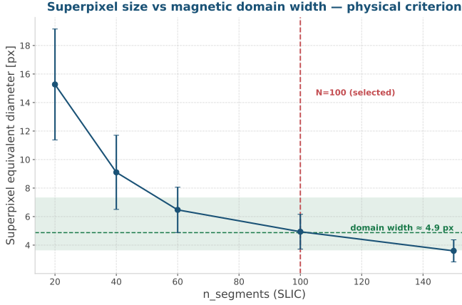
Figure 23: Physical criterion for the SLIC segmentation used by the perturbation-based baselines. The superpixel equivalent diameter is plotted against the number of SLIC segments; the selected value N = 100 (dashed red) yields superpixels whose size matches the characteristic magnetic domain width ( \approx 4.9 px, dashed green), so that each interpretable region corresponds to a single magnetic domain.
