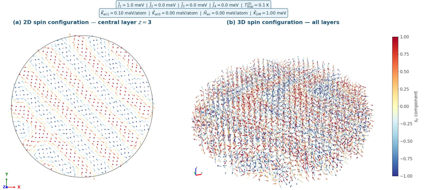
Figure 11: Converged ground-state spin configuration of a representative magnetic nanodot at T_{final}^{(0)} = 0.1 K under a fixed parameter configuration. (a) Two-dimensional projection of the out-of-plane magnetization field s_z : colored dots indicate spins oriented predominantly out-of-plane, while colored arrows represent the in-plane orientation (s_x, s_y) of transverse moments. (b) Full three-dimensional spin configuration, revealing the volumetric coherence of the labyrinthine chiral domain structure stabilized by the competition between \tilde{J}_1 and \tilde{K}_{DM} . Color encodes the s_z component.
