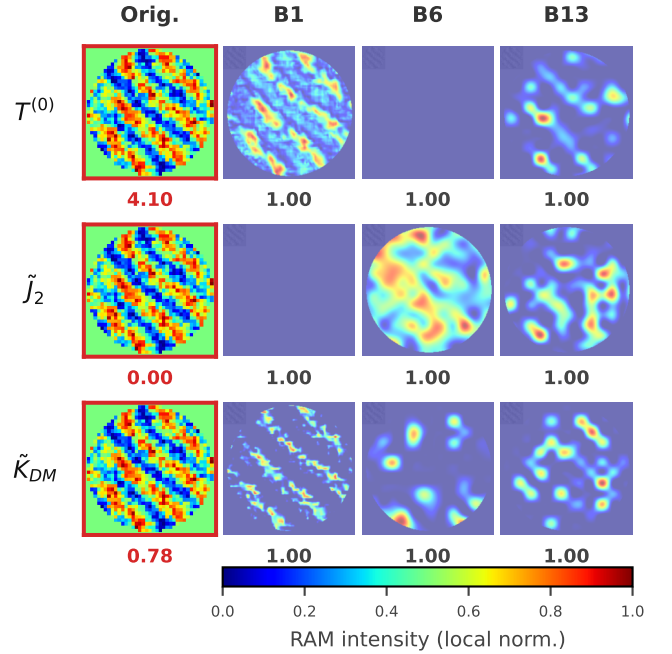
Figure 9: RAMs \tilde{\mathcal{R}}_{\text{RAM}}^{(l,p)} for the Xception architecture in the helical phase. Rows are three Hamiltonian parameters \{T^{(0)}, \tilde{J}_2, \tilde{K}_{DM}\} ; columns are three representative network layers— block1 (entry, B1), block6 (middle, B6), and block13 (exit, B13)—with the original s_z image in the leftmost column. Each panel overlays the RAM intensity (locally normalized) on the magnetization; the value below each original image is the ground-truth parameter.
