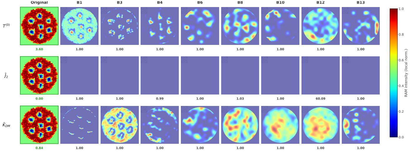
Figure 15: RAMs \tilde{\mathcal{K}}_{\text{RAM}}^{(l,p)} for the Xception architecture in the skyrmion phase. Rows are three Hamiltonian parameters \{T^{(0)}, \tilde{J}_2, \tilde{K}_{DM}\} ; columns are network layers from block1 (entry, 112 \times 112 ) to block13 (exit, 14 \times 14 ), with the original s_z image in the leftmost column. Each panel overlays the RAM (jet colormap) on the magnetization, locally normalized per layer. The score below each cell is the fraction of activation within the nanodot disk; the value below each original image is the ground-truth parameter.
