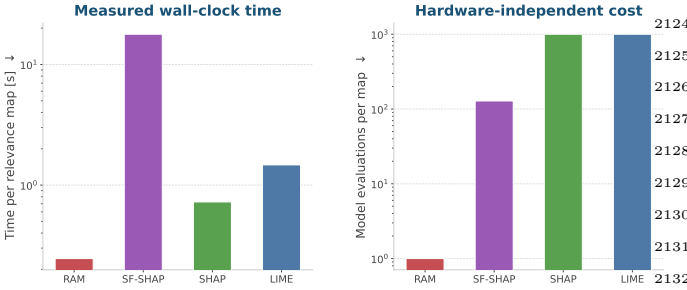
Figure 20: Computational cost of the interpretability methods. Left: measured wall-clock time per relevance map (log scale). Right: number of model evaluations per map (log scale). A RAM requires a single backward pass, against \sim 10^3 evaluations for LIME and SHAP and 128 for SF-SHAP.
