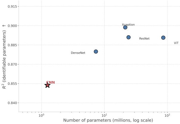
Figure 7: Mean R^2 over the identifiable Hamiltonian parameters versus the number of trainable weights (log scale) for the five architectures. The nearly flat trend—the compact CNN already matching models two orders of magnitude larger—indicates that accuracy is limited by the physical information in the s_z projection, not by model capacity.
