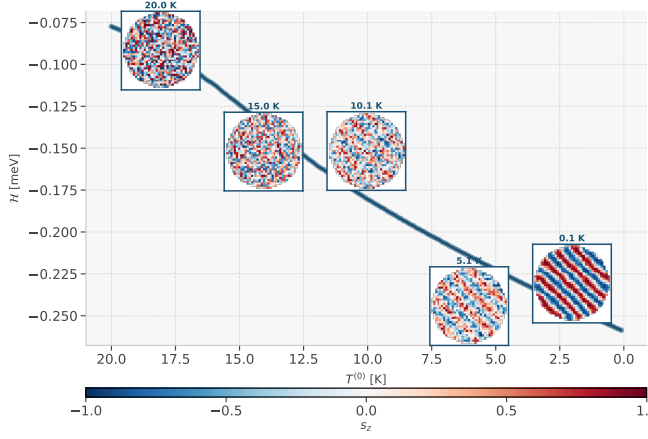
Figure 5: Thermodynamic convergence of a representative nanodot during simulated annealing. The main panel shows the total Hamiltonian energy \mathcal{H} [meV] versus the annealing temperature T^{(0)} [K]; each inset shows the s_z field of the central layer at that state, tracing the transition from a disordered paramagnetic phase at high T^{(0)} to a relaxed labyrinthine configuration at T^{(0)} = 0.1 K.
