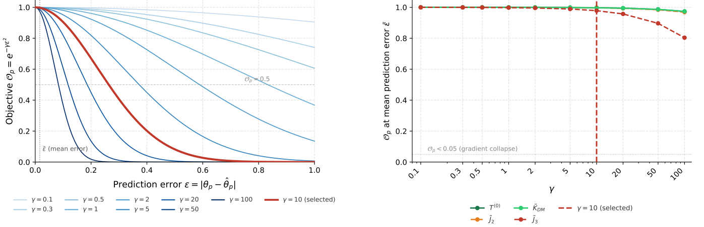
Figure 14: Sensitivity analysis of the RAM precision factor \gamma . Left: shape of the Gaussian objective O_p = e^{-\gamma \epsilon^2} versus the prediction error \epsilon = |\theta_p - \hat{\theta}_p| for \gamma \in \{0.1, \dots, 100\} (selected \gamma = 10 in red; vertical dotted line = empirical mean error). Right: O_p evaluated at each parameter’s mean error as a function of \gamma ; the horizontal dotted line marks the gradient-collapse threshold O_p = 0.05 . The value \gamma = 10 is the selected operating point.
