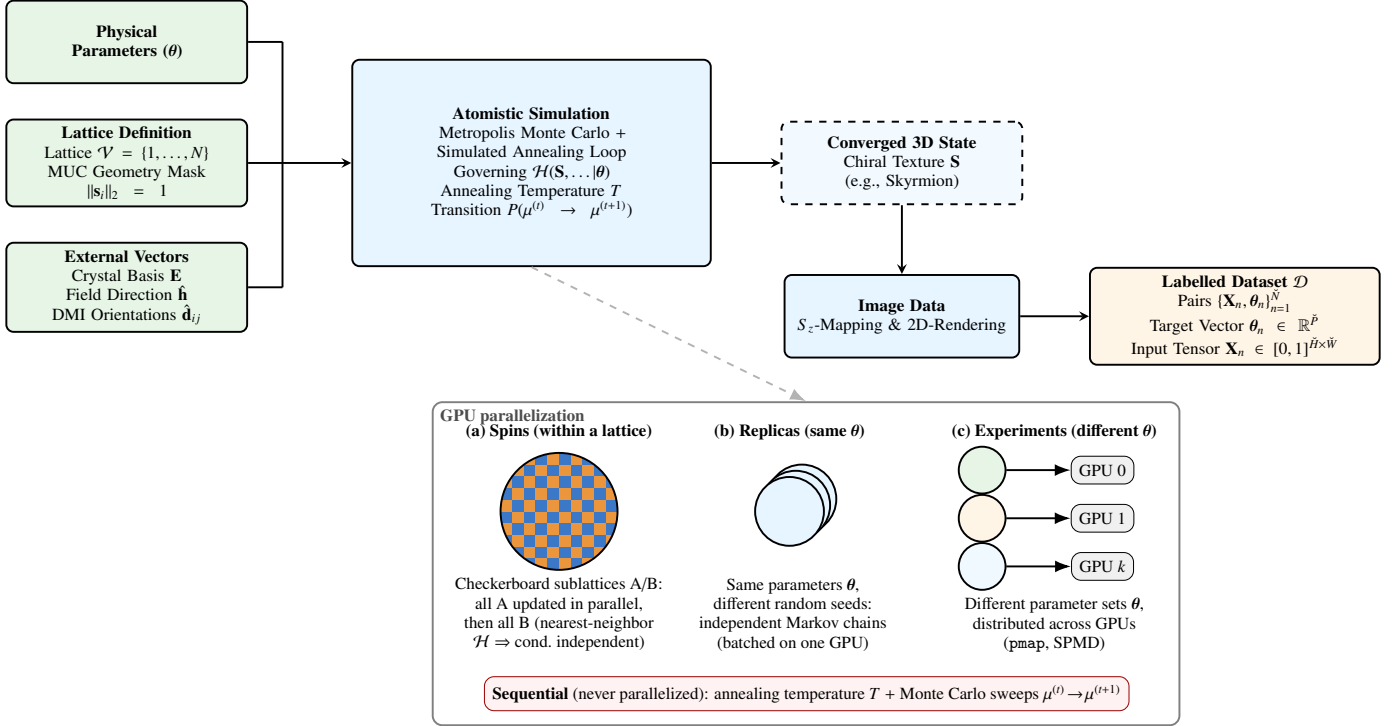
Figure 1: Flowchart of the GPU-accelerated image-based magnetic dataset generation. Foundational inputs (green), the Hamiltonian parameters \theta , the unit-cell geometry, and the external directional vectors, drive the atomistic Metropolis Monte Carlo simulation with simulated annealing (blue), relaxing the system into a converged 3D topological state. The resulting vector field is then projected, rendered, and preprocessed (yellow) into the labelled dataset \mathcal{D} mapping 2D s_z images to their generating parameters. The bottom inset details the three levels of GPU parallelization: (a) spins , within a single lattice, the nearest-neighbor Hamiltonian makes the two checkerboard sublattices A/B conditionally independent, so all sites of one sublattice are updated simultaneously (with the other held fixed) before switching, reproducing a sequential sweep; (b) replicas , the same parameter set \theta is run with different random seeds as independent Markov chains, batched on a GPU; and (c) experiments : different parameter sets \theta are distributed across GPUs via single-program multiple-data (pmap, SPMD). The annealing temperature and the Monte Carlo sweeps \mu^{(t)} \rightarrow \mu^{(t+1)} remain strictly sequential, so the parallelization introduces no approximation to the underlying physics.
