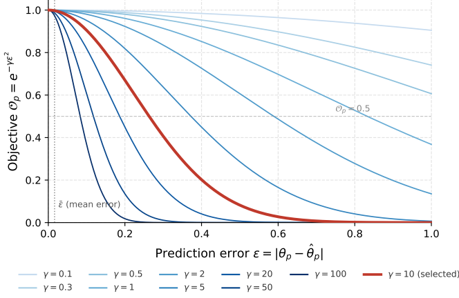
Figure 8: Sensitivity analysis of the RAM precision factor \gamma . Left: shape of the Gaussian objective O_p = e^{-\gamma \epsilon^2} versus the prediction error \epsilon = |\theta_p - \hat{\theta}_p| for \gamma \in \{0.1, \dots, 100\} (selected \gamma = 10 in red; vertical dotted line = empirical mean error). Right: O_p evaluated at each parameter’s mean error as a function of \gamma ; the horizontal dotted line marks the gradient-collapse threshold O_p = 0.05 . The value \gamma = 10 is the selected operating point.
