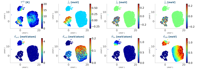
Figure 6: UMAP-based 2D projection of the Xception latent space on the held-out test set, colored by each of the eight Hamiltonian parameters \theta = [T^{(0)}, \tilde{J}_1, \tilde{J}_2, \tilde{J}_3, \tilde{J}_4, \tilde{K}_{an1}, \tilde{K}_{anS}, \tilde{H}_{ex}, \tilde{K}_{DM}] . Each point represents a magnetization image \mathbf{X}_n projected from the high-dimensional feature space of the Xception backbone into two dimensions via UMAP.
