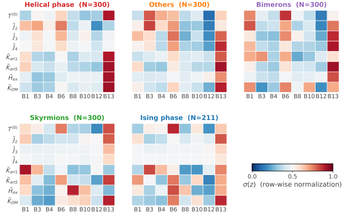
Figure 10: Heatmap of the mean maximum RAM activation per network layer (columns, B1–B13) and Hamiltonian parameter \theta (rows), for the five magnetic phases, averaged over N = 300 test samples per phase ( N = 211 for Ising; Xception CNN) and measured within the nanodot disk (masked RAM). Activations are normalized row-wise (per parameter, across layers) via a sigmoid \sigma(\frac{z-\mu}{\sigma_x}) , so warm cells mark the layers where each parameter’s gradient response is relatively strongest. The identifiable parameters peak at the exit-flow layer B13, whereas \tilde{J}_3 and \tilde{J}_4 show a flat, unstructured profile with no dominant layer.
