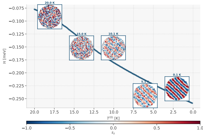
Figure 3: Thermodynamic convergence of a representative nanodot during simulated annealing. The main panel shows the total Hamiltonian energy \mathcal{H} [meV] versus the annealing temperature T^{(0)} [K]; each inset shows the s_z field of the central layer at that state, tracing the transition from a disordered paramagnetic phase at high T^{(0)} to a relaxed labyrinthine configuration at T^{(0)} = 0.1 K.
