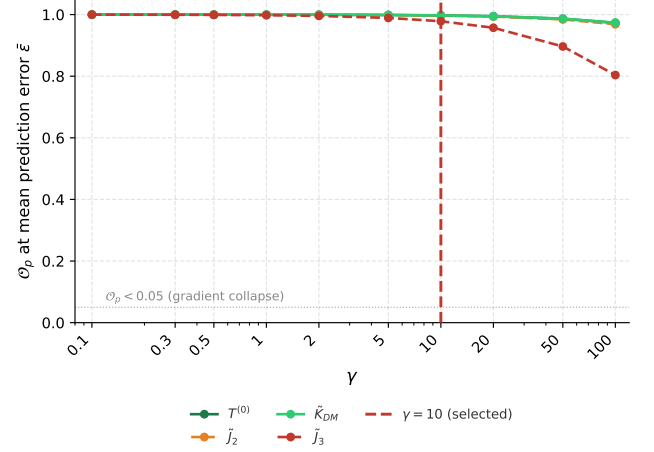
Figure 8: Sensitivity analysis of the RAM precision factor \gamma . Left: shape of the Gaussian objective O_p = e^{-\gamma \epsilon^2} versus the prediction error \epsilon = |\theta_p - \hat{\theta}_p| for \gamma \in \{0.1, \dots, 100\} (selected \gamma = 10 in red; vertical dotted line = empirical mean error). Right: O_p evaluated at each parameter’s mean error as a function of \gamma ; the horizontal dotted line marks the gradient-collapse threshold O_p = 0.05 . The value \gamma = 10 is the selected operating point.
