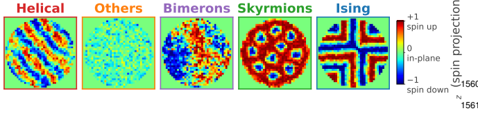
Figure 7: Representative magnetization image \mathbf{X}_n for each of the five magnetic phase categories identified by clustering the Xception latent space (the sample nearest the cluster centroid in the UMAP embedding); color encodes the out-of-plane component m_z (+1 spin up, -1 spin down). The phases span ordered helical stripes, thermally disordered others , mixed-chirality bimerons, dense skyrmion lattices, and sharp Ising domain walls.
