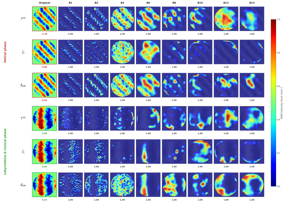
Figure 20: RAMs \tilde{\mathcal{R}}_{\text{RAM}}^{(l,p)} for the Xception architecture, shown for the two most topologically structured magnetic phases — Helical and Labyrinthine & Conical — selected as the most representative cases from the full four-phase RAM computation. Three Hamiltonian parameters \{T^{(0)}, J_2, \tilde{K}_{DM}\} are shown. Each panel displays the RAM overlay (jet colormap) on the original s_z magnetization image (grayscale), with local per-cell normalization to reveal spatial attribution patterns at each layer independently. Rows correspond to phase–parameter pairs; columns correspond to network layers from block1 (entry, 112 \times 112 ) to block13 (exit, 14 \times 14 ). The numerical score below each RAM cell reports the fraction of activation concentrated within the nanodot disk boundary, and the value below each original image reports the ground-truth parameter value for that representative sample. A physically consistent hierarchical decoupling is observed: early layers capture fine-grained domain periodicity while deeper layers consolidate activations into topologically significant spatial hotspots.
