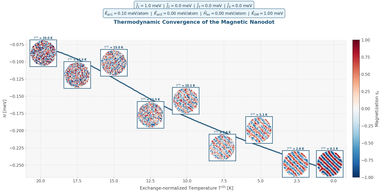
Figure 9: Thermodynamic convergence of a representative magnetic nanodot during simulated annealing. The main panel shows the total Hamiltonian energy \mathcal{H} [meV] as a function of the exchange-normalized annealing temperature T^{(0)} [K] under the fixed parameter configuration. Each inset depicts the two-dimensional out-of-plane magnetization field s_z of the central layer at the corresponding thermal state, illustrating the progressive transition from a fully disordered paramagnetic phase at high T^{(0)} to a thermodynamically relaxed labyrinthine domain configuration at T^{(0)} = 0.1 K, driven by the competing energetic contributions of \tilde{J}_1 and \tilde{K}_{DM} .
