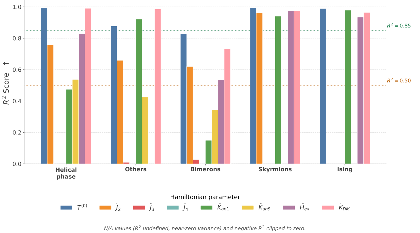
Figure 17: Per-phase R^2 score of the best-performing model, Xception, across all eight Hamiltonian parameters \theta for the five identified magnetic phase categories. Each bar group corresponds to one magnetic phase and each bar to one target parameter. Dashed horizontal lines mark the identifiability thresholds at R^2 = 0.85 (high predictability) and R^2 = 0.50 (partial predictability). Negative R^2 values and near-zero variance cases (N/A) are clipped to zero. The Skyrmion and Ising phases achieve near-perfect accuracy across the identifiable parameters, while the Bimeron and Others phases exhibit the lowest identifiability owing to their weakly discriminative, structurally ambiguous magnetization textures.
