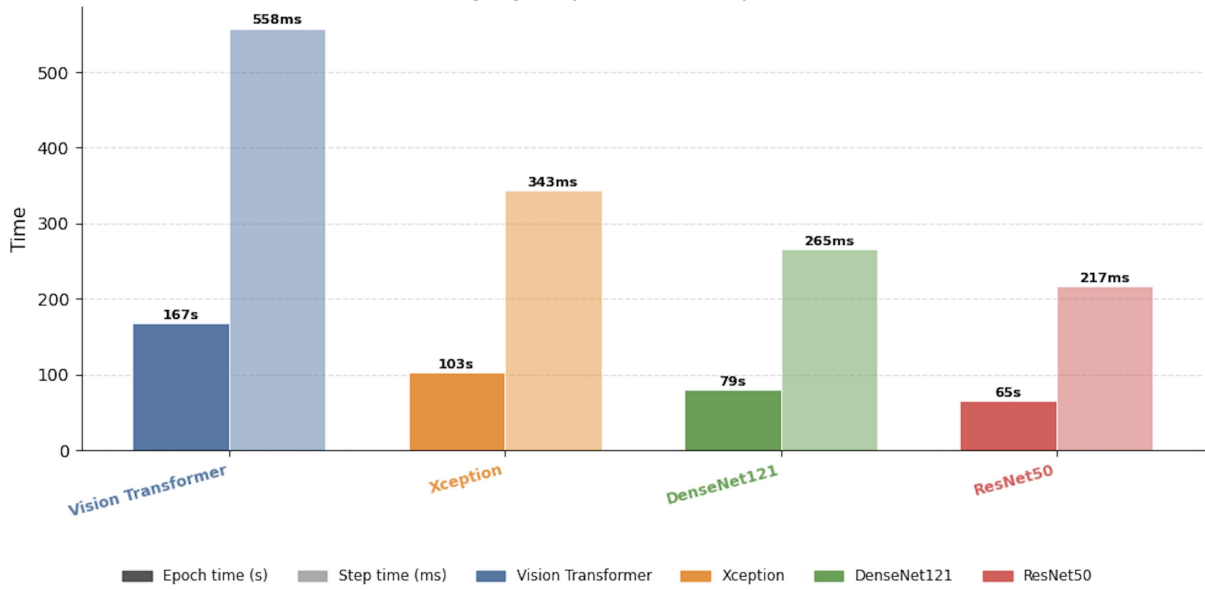
Figure 24: Training computational cost comparison across the four regression architectures on an NVIDIA H100 GPU (Google Colab Pro). (a) Wall-clock time per epoch in the stable warm-start regime. (b) Per-step gradient update time (299 steps/epoch, batch size B = 512 ). The Vision Transformer incurs the highest training cost (167 s/epoch, 558 ms/step) due to its 85.8M-parameter self-attention architecture, while ResNet50 achieves the fastest throughput (65 s/epoch, 217 ms/step). The training cost hierarchy directly reflects the architectural complexity of each model.
