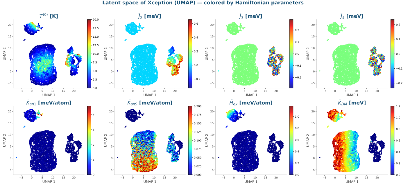
Figure 14: UMAP-based 2D projection of the Xception latent space on the held-out test set, colored by each of the eight Hamiltonian parameters \theta = [T^{(0)}, \tilde{J}_2, \tilde{J}_3, \tilde{J}_4, \tilde{K}_{an1}, \tilde{K}_{anS}, \tilde{H}_{ex}, \tilde{K}_{DM}] . Each point represents a magnetization image \mathbf{X}_n projected from the high-dimensional feature space of the Xception backbone into two dimensions via UMAP.
