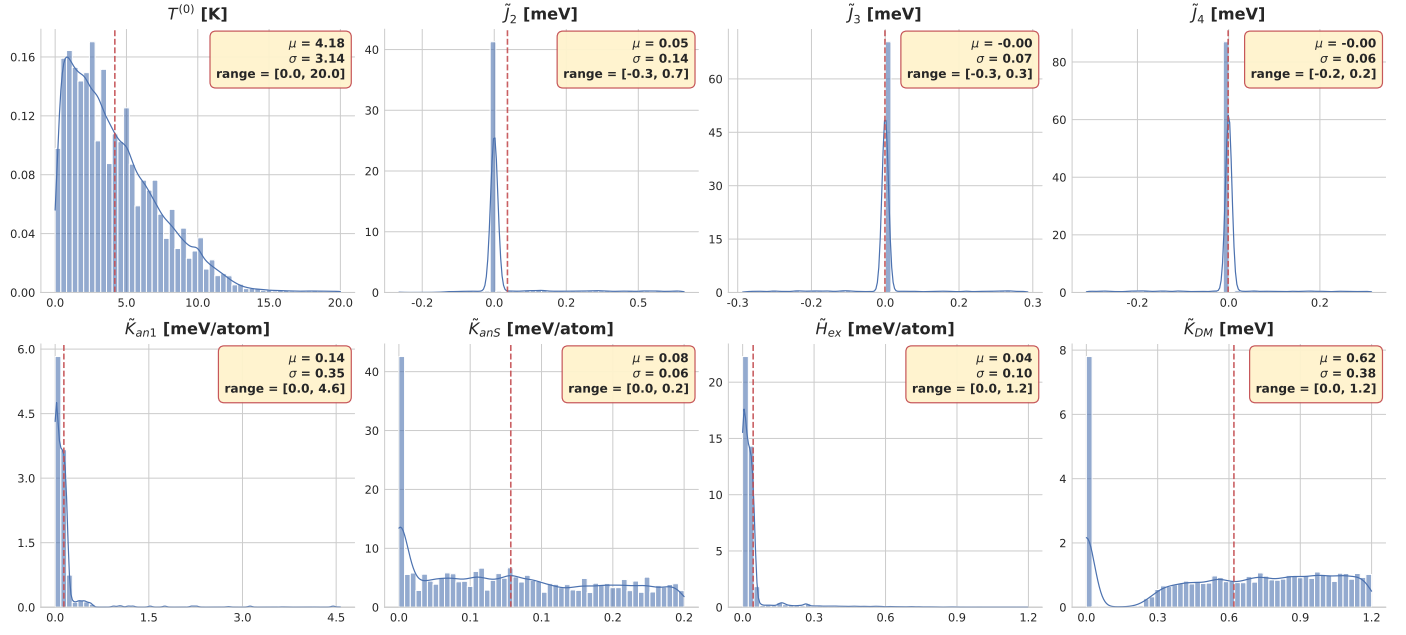
Figure 8: Empirical distributions of the thermodynamic and Hamiltonian parameters \{T^{(0)}, \tilde{J}_2, \tilde{J}_3, \tilde{J}_4, \tilde{K}_{an1}, \tilde{K}_{ans}, \tilde{H}_{ex}, \tilde{K}_{DM}\} used to generate the dataset. Each subplot presents a histogram and KDE for a given variable, along with summary statistics including mean, standard deviation, and value range.
