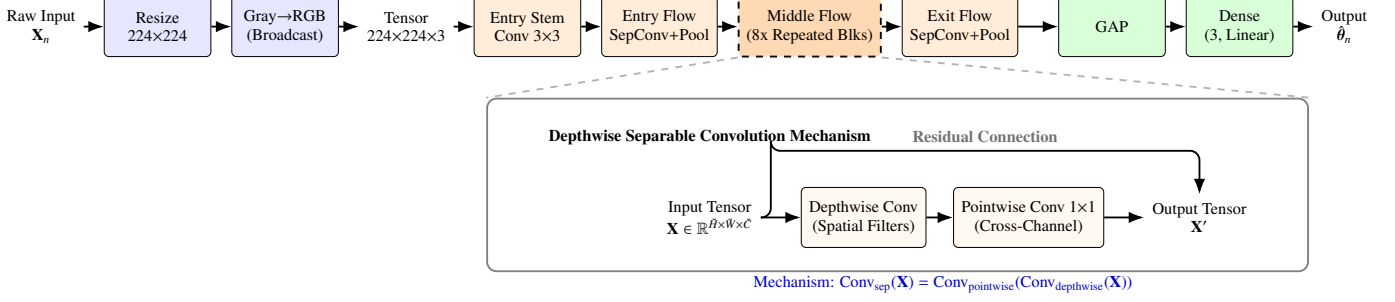
Figure 5: Xception architecture pipeline for Hamiltonian parameter estimation. The feature extractor composed of Entry, Middle, and Exit flows. A detailed horizontal view illustrates the depthwise separable convolution mechanism where spatial feature extraction (depthwise) and cross-channel correlations (pointwise) are entirely decoupled. The final aggregated features are mapped to physical constants.
