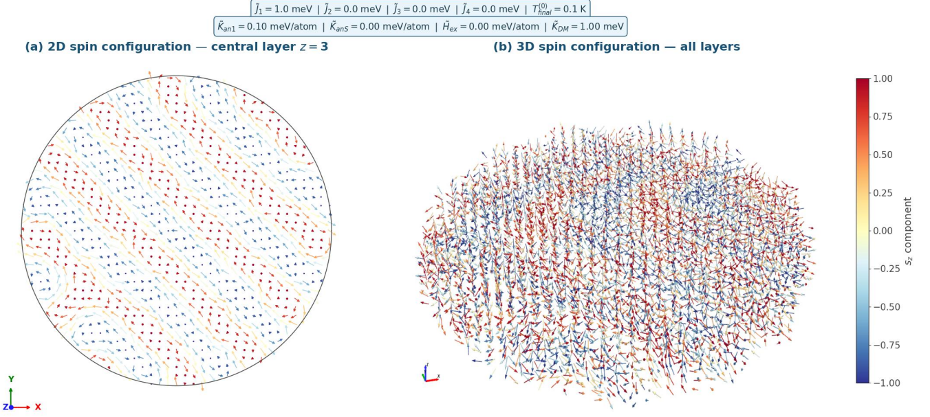
Figure 10: Converged ground-state spin configuration of a representative magnetic nanodot at T_{\text{final}}^{(0)} = 0.1 \text{ K} under a fixed parameter configuration. (a) Two-dimensional projection of the out-of-plane magnetization field s_z : colored dots indicate spins oriented predominantly out-of-plane, while colored arrows represent the in-plane orientation ( s_x, s_y ) of transverse moments. (b) Full three-dimensional spin configuration, revealing the volumetric coherence of the labyrinthine chiral domain structure stabilized by the competition between \bar{J}_1 and \tilde{K}_{DM} . Color encodes the s_z component.
