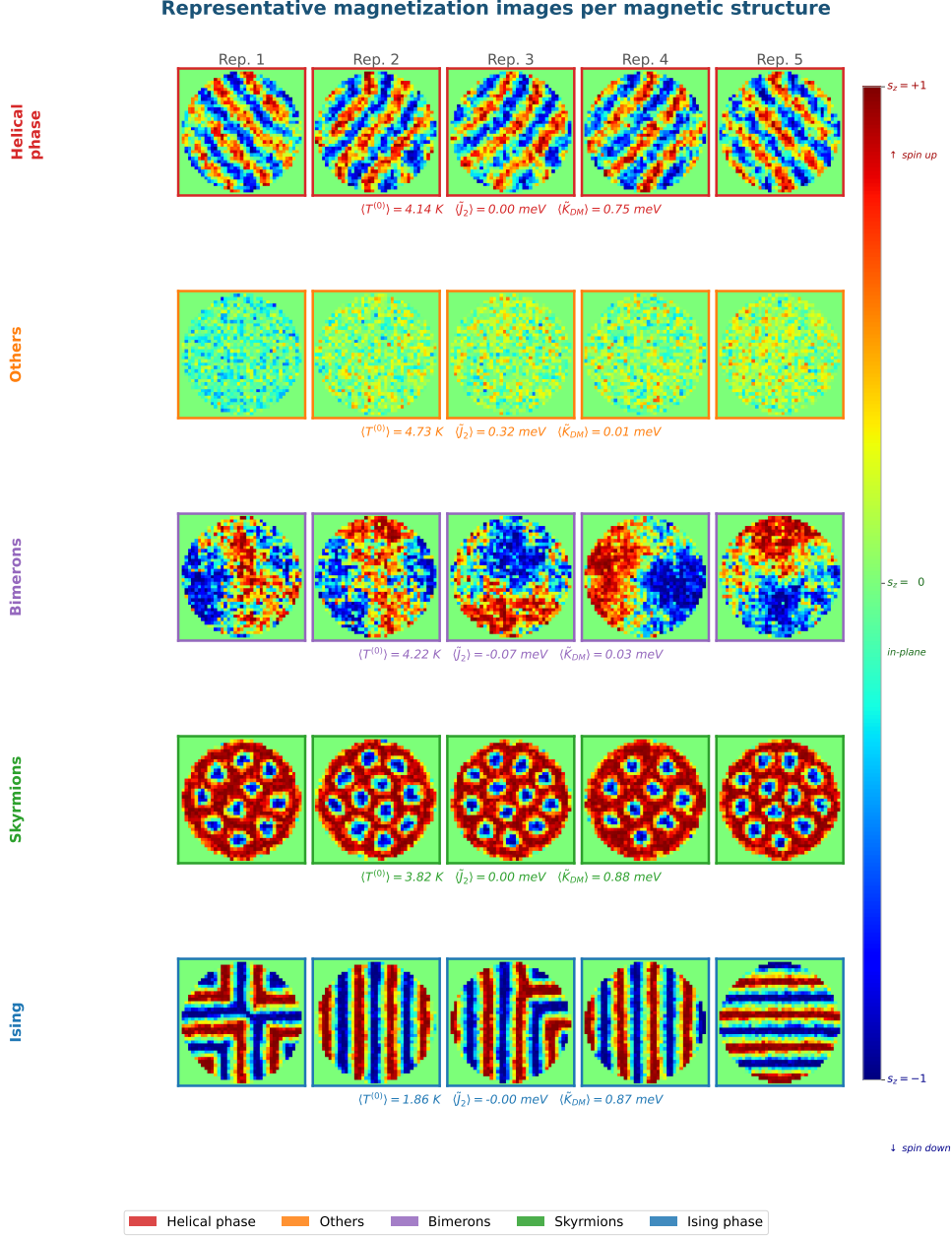
Figure 16: Representative magnetization images \mathbf{X}_n for each of the five magnetic phase categories identified through clustering of the Xception latent space. Each row displays five samples selected as the nearest neighbors to the cluster centroid in the UMAP embedding. Mean Hamiltonian parameters \langle T^{(0)} \rangle , \langle J_2 \rangle , and \langle K_{DM} \rangle are reported below each row. The Helical phase presents ordered, spatially coherent stripe and labyrinthine configurations with consistent periodicity and chiral winding. The Others category gathers thermally disordered, transitional, and topologically mixed configurations that lack a defining spatial signature. The Bimeron phase shows mixed-chirality textures with coexisting in-plane and out-of-plane components forming irregular domains. The Skyrmion phase displays dense lattices of isolated, radially symmetric topological solitons stabilized by a strong DMI. The Ising phase exhibits sharp, discrete domain walls between collinear up/down regions, characteristic of the high-anisotropy regime.
