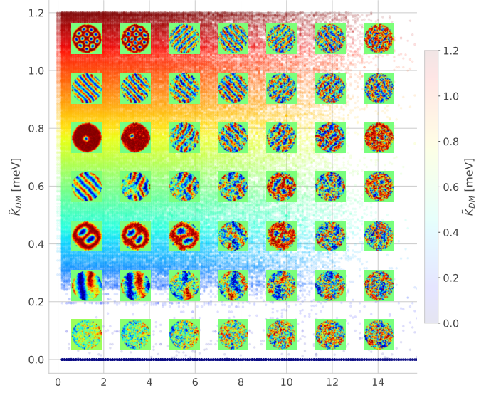
Figure 4: Two-dimensional phase diagram of the magnetization texture \mathbf{X}_n as a function of the annealing temperature T^{(0)} and the DMI strength \tilde{K}_{DM} . Each cell shows an enlarged representative image on a coarse sampling grid; the background color encodes \tilde{K}_{DM} .
