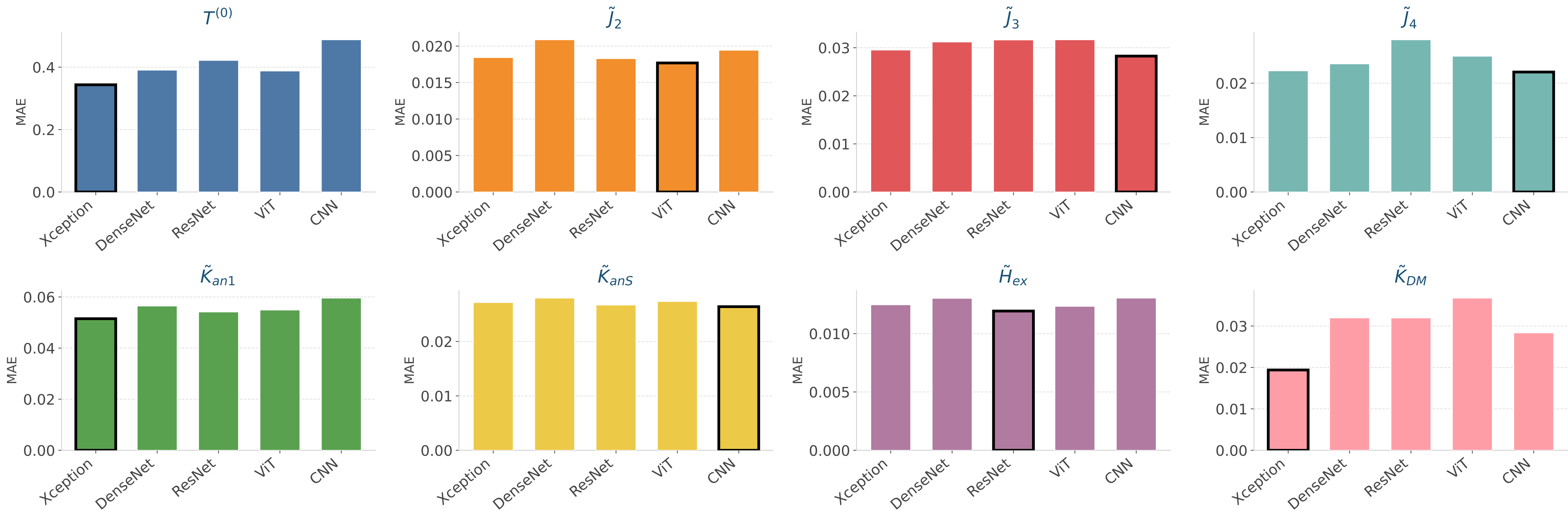
Each subplot uses its own scale (units differ: T^{(0)} in K, others in meV). Best model per variable outlined in black.
