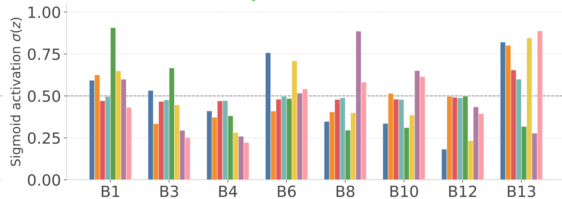
Skymions (N=300)
