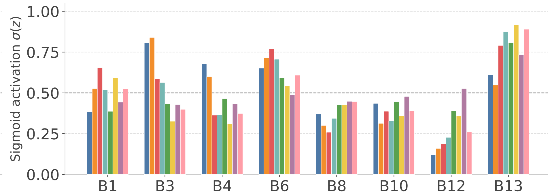
Skymions (N=300)
