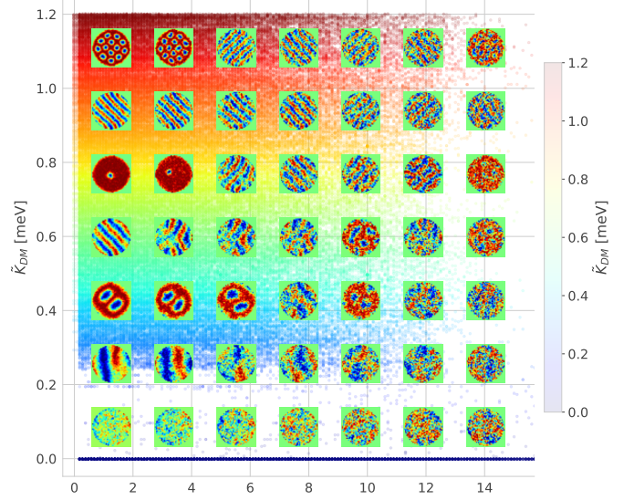
Figure 4: Two-dimensional phase diagram of the magnetization texture \mathbf{X}_r as a function of the annealing temperature T^{(0)} and the DMI strength \tilde{K}_{DM} . Each cell shows an enlarged representative image on a coarse sampling grid; the background color encodes \tilde{K}_{DM} .
