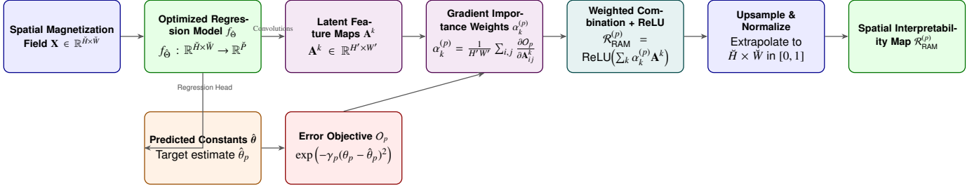
Figure 2: RAMs extraction pipeline. Latent feature maps and continuous predictions from the network backbone are explicitly coupled via an error-decay objective. Gradient-based importance weights combine these features to produce a normalized, physically traceable spatial saliency map for the target Hamiltonian parameter \theta_p .
