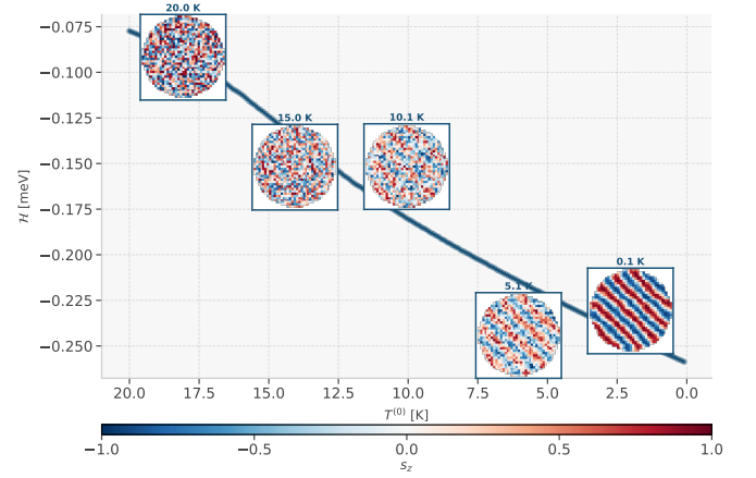
Figure 3: Thermodynamic convergence of a representative nanodot during simulated annealing. The main panel shows the total Hamiltonian energy \mathcal{H} [meV] versus the annealing temperature T^{(0)} [K]; each inset shows the s_z field of the central layer at that state, tracing the transition from a disordered paramagnetic phase at high T^{(0)} to a relaxed labyrinthine configuration at T^{(0)} = 0.1 K.
