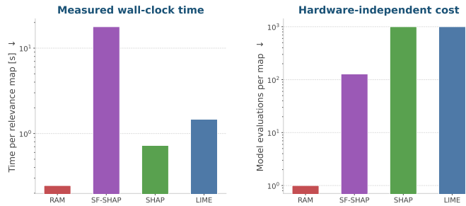
Figure 13: Computational cost of the interpretability methods. Left: measured wall-clock time per relevance map (log scale). Right: number of model evaluations per map (log scale). A RAM requires a single backward pass, against \sim 10^3 evaluations for LIME and SHAP and 128 for SF-SHAP.
