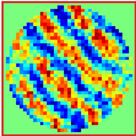
Helical
