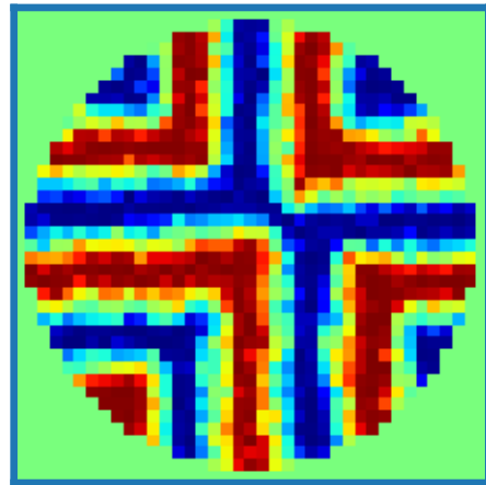
Ising
