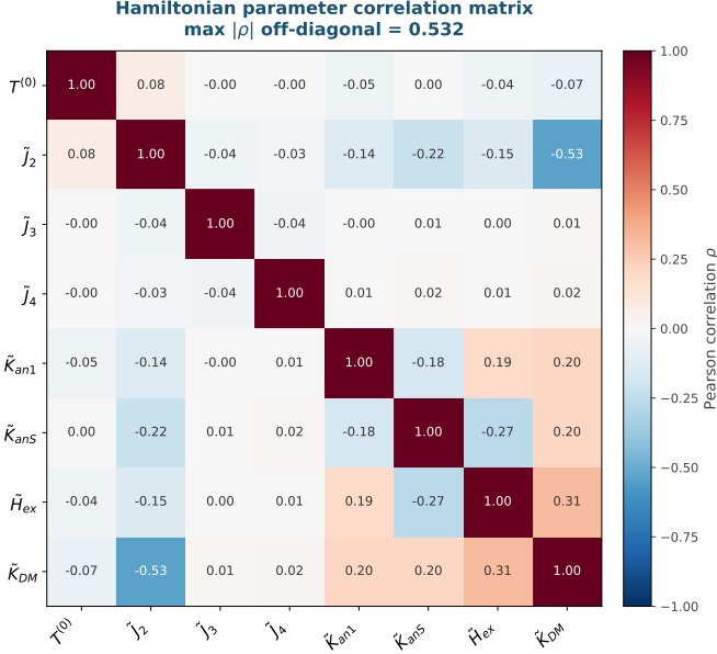
Figure 8: Pairwise Pearson correlation matrix of the eight Hamiltonian parameters computed over the entire dataset of 166,141 configurations. All parameter pairs are essentially uncorrelated ( |\rho| \lesssim 0.3 ), with the single exception of the second-shell exchange \tilde{J}_2 and the DMI strength \tilde{K}_{DM} ( \rho \approx -0.53 ), whose anti-correlation is a direct consequence of the deliberate design in which the exchange-frustration and chiral mechanisms are activated in a mutually exclusive fashion. The absence of spurious cross-parameter correlations indicates that the model cannot exploit artificial statistical shortcuts to infer one parameter from another.
