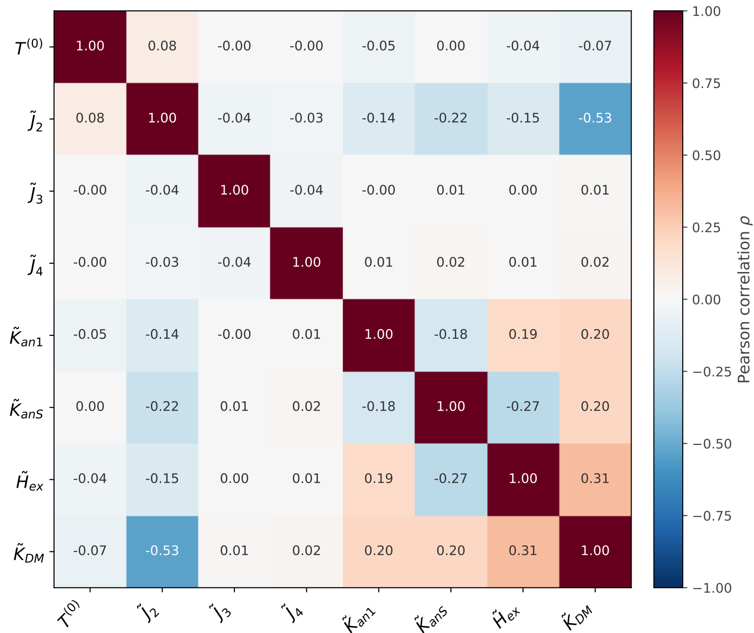
Hamiltonian parameter correlation matrix max |\rho| off-diagonal = 0.532
