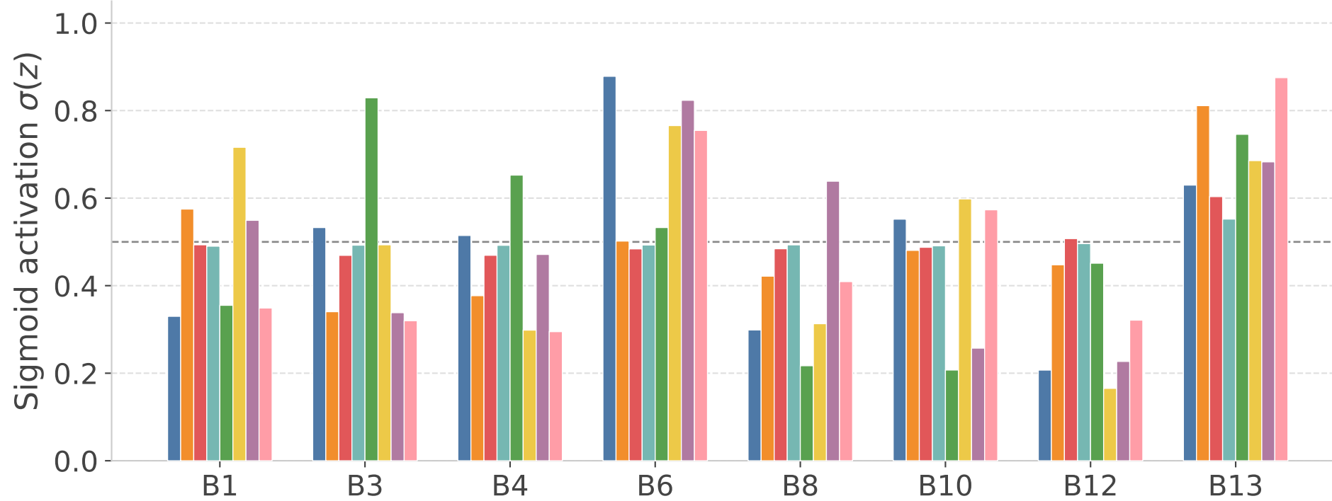
Ising phase (N=211)
