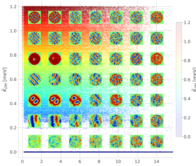
Figure 4: Two-dimensional phase diagram of the magnetization texture \mathbf{X}_n as a function of the annealing temperature T^{(0)} and the DMI strength \tilde{K}_{DM} . Each cell shows an enlarged representative image on a coarse sampling grid; the background color encodes \tilde{K}_{DM} .
