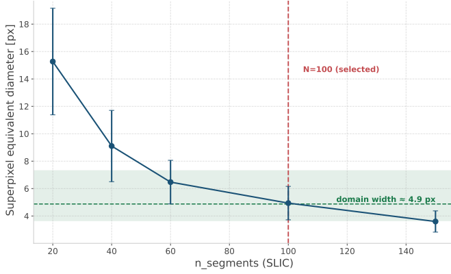
Figure 11: Physical criterion for the SLIC segmentation used by the perturbation-based baselines. The superpixel equivalent diameter is plotted against the number of SLIC segments; the selected value N = 100 (dashed red) yields superpixels whose size matches the characteristic magnetic domain width ( \approx 4.9 px, dashed green), so that each interpretable region corresponds to a single magnetic domain.
