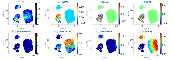
Figure 6: UMAP-based 2D projection of the Xception latent space on the held-out test set, colored by each of the eight Hamiltonian parameters \theta = [T^{(0)}, \tilde{J}_2, \tilde{J}_3, \tilde{J}_4, \tilde{K}_{anS}, \tilde{K}_{an1}, \tilde{H}_{ex}, \tilde{K}_{DM}] . Each point represents a magnetization image \mathbf{X}_n projected from the high-dimensional feature space of the Xception backbone into two dimensions via UMAP.
