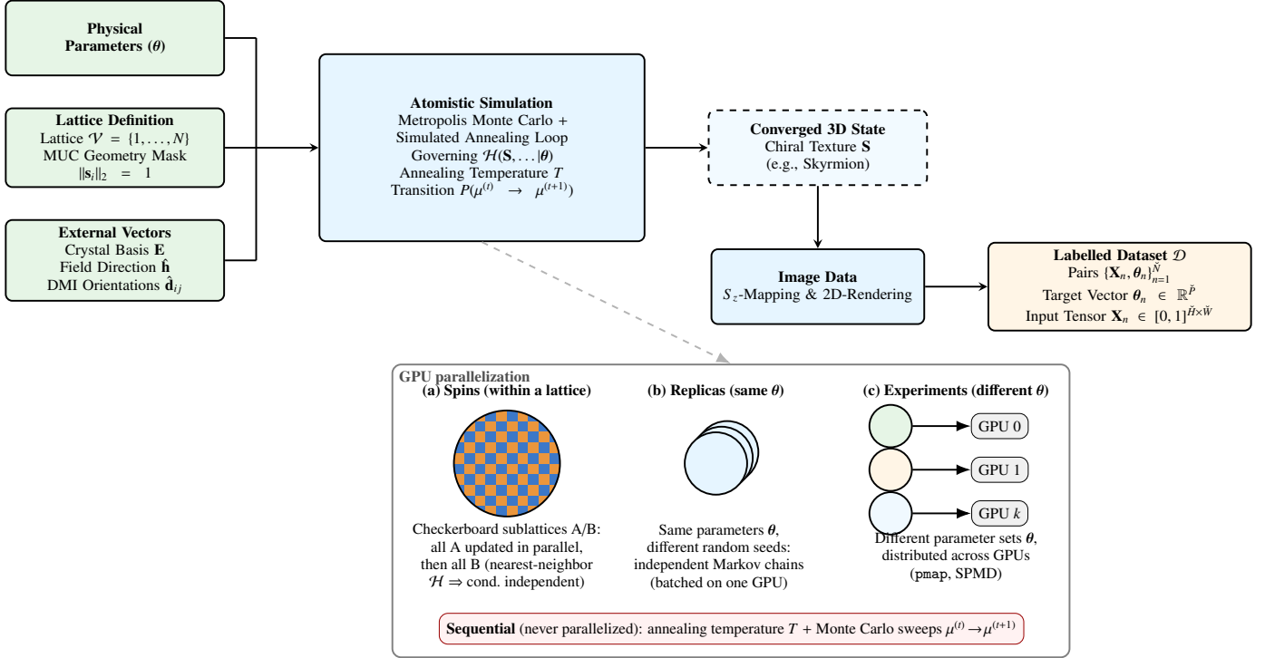
Figure 1: Flowchart of the image-based magnetic dataset generation. Foundational inputs (green)—the Hamiltonian parameters \theta , the unit-cell geometry, and the external directional vectors—drive the atomistic Metropolis Monte Carlo simulation with simulated annealing (blue), which relaxes the system into a converged 3D topological state. The resulting vector field is then projected, rendered, and preprocessed (yellow) into the labelled dataset \mathcal{D} mapping 2D s_z images to their generating parameters. The bottom inset details the three levels of GPU parallelization of the Monte Carlo loop: (a) spins —within a single lattice, the nearest-neighbor Hamiltonian makes the two checkerboard sublattices A/B conditionally independent, so all sites of one sublattice are updated simultaneously (with the other held fixed) before switching, exactly reproducing a sequential sweep; (b) replicas —the same parameter set \theta is run with different random seeds as independent Markov chains, batched on a GPU; and (c) experiments —different parameter sets \theta are distributed across GPUs via single-program multiple-data (pmap) execution. Crucially, the annealing temperature and the Monte Carlo sweeps \mu^{(t)} \rightarrow \mu^{(t+1)} remain strictly sequential, so the parallelization introduces no approximation to the underlying physics.
