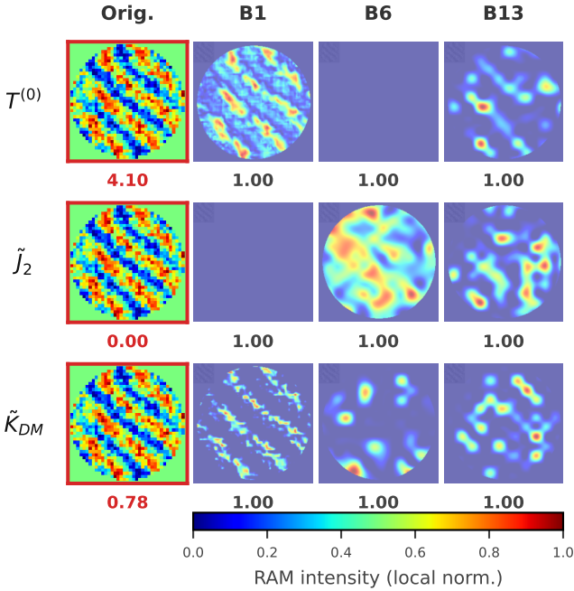
Figure 9: RAMs \tilde{\mathcal{R}}_{\text{RAM}}^{(L,p)} for the Xception architecture in the helical phase. Rows 1800 are three Hamiltonian parameters \{T^{(0)}, \tilde{J}_2, \tilde{K}_{DM}\} ; columns are three representa 1801 tive network layers—block1 (entry, B1), block6 (middle, B6), and block13 1802 (exit, B13)—with the original s_z image in the leftmost column. Each pane 1803 l overlays the RAM intensity (locally normalized) on the magnetization; the value 1804 below each original image is the ground-truth parameter.
