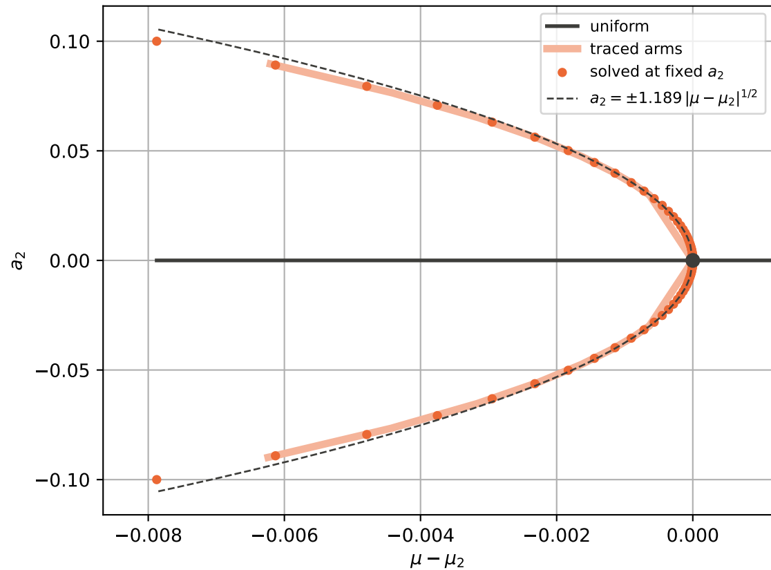
Pitchfork at \mu_2 = 0.383445 , fitted exponent 0.5000
