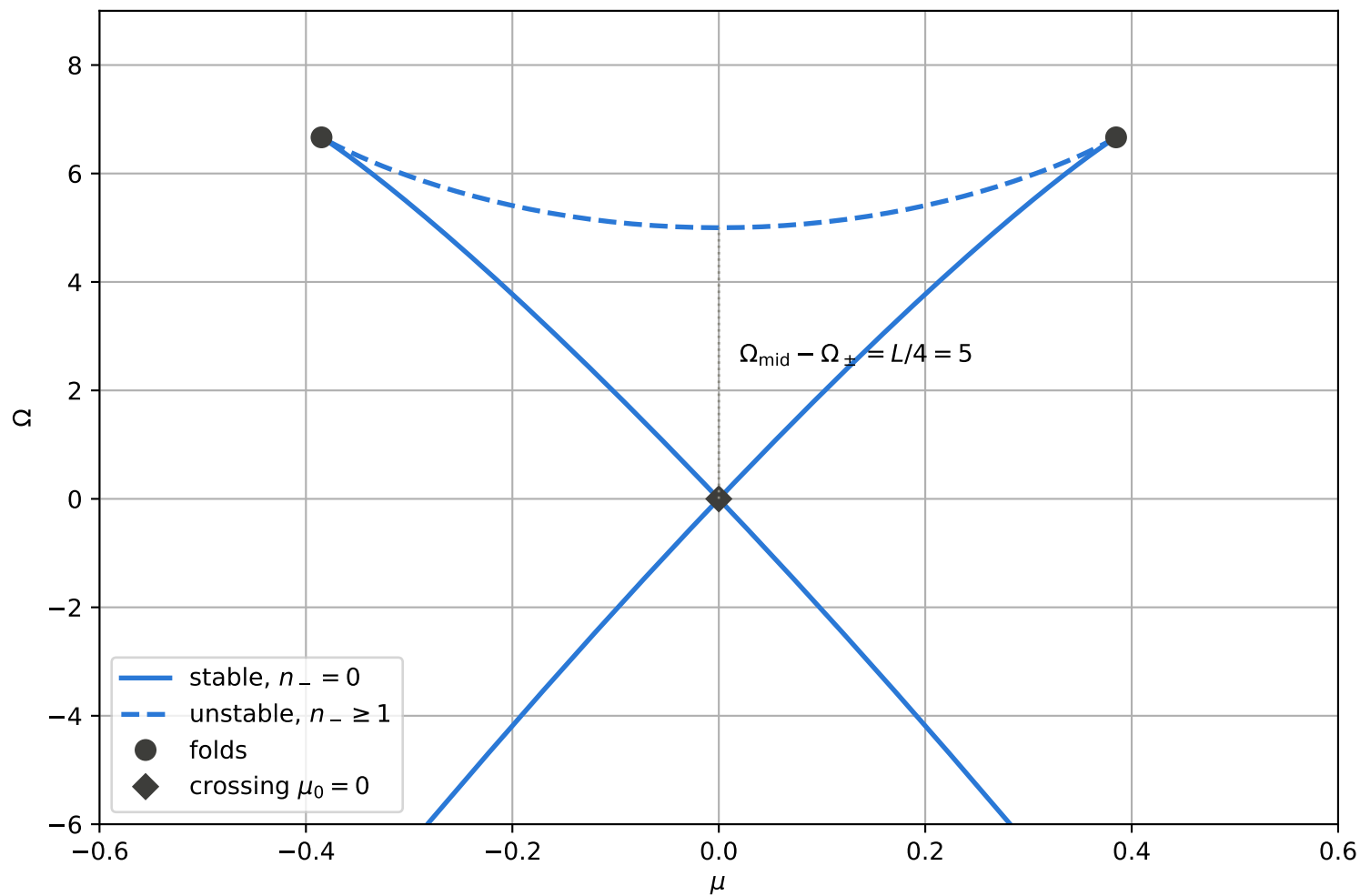
Uniform branch: the swallowtail
