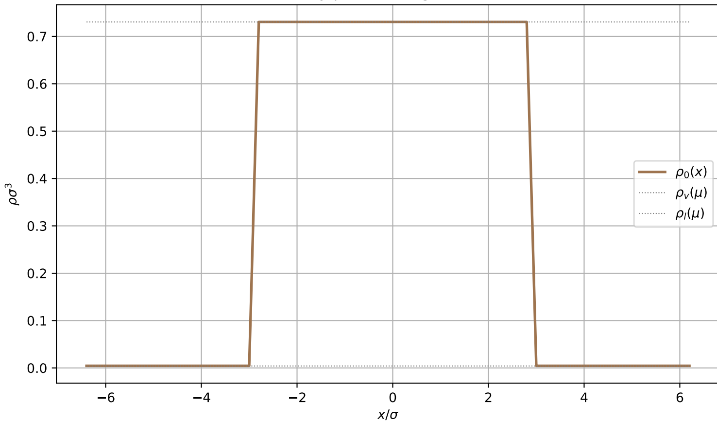
Initial density profile along x [WhiteBearII]
