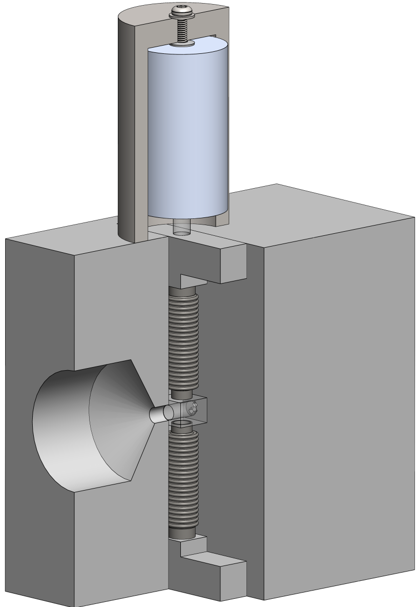
Figure 3: PTCD Full Assembly
