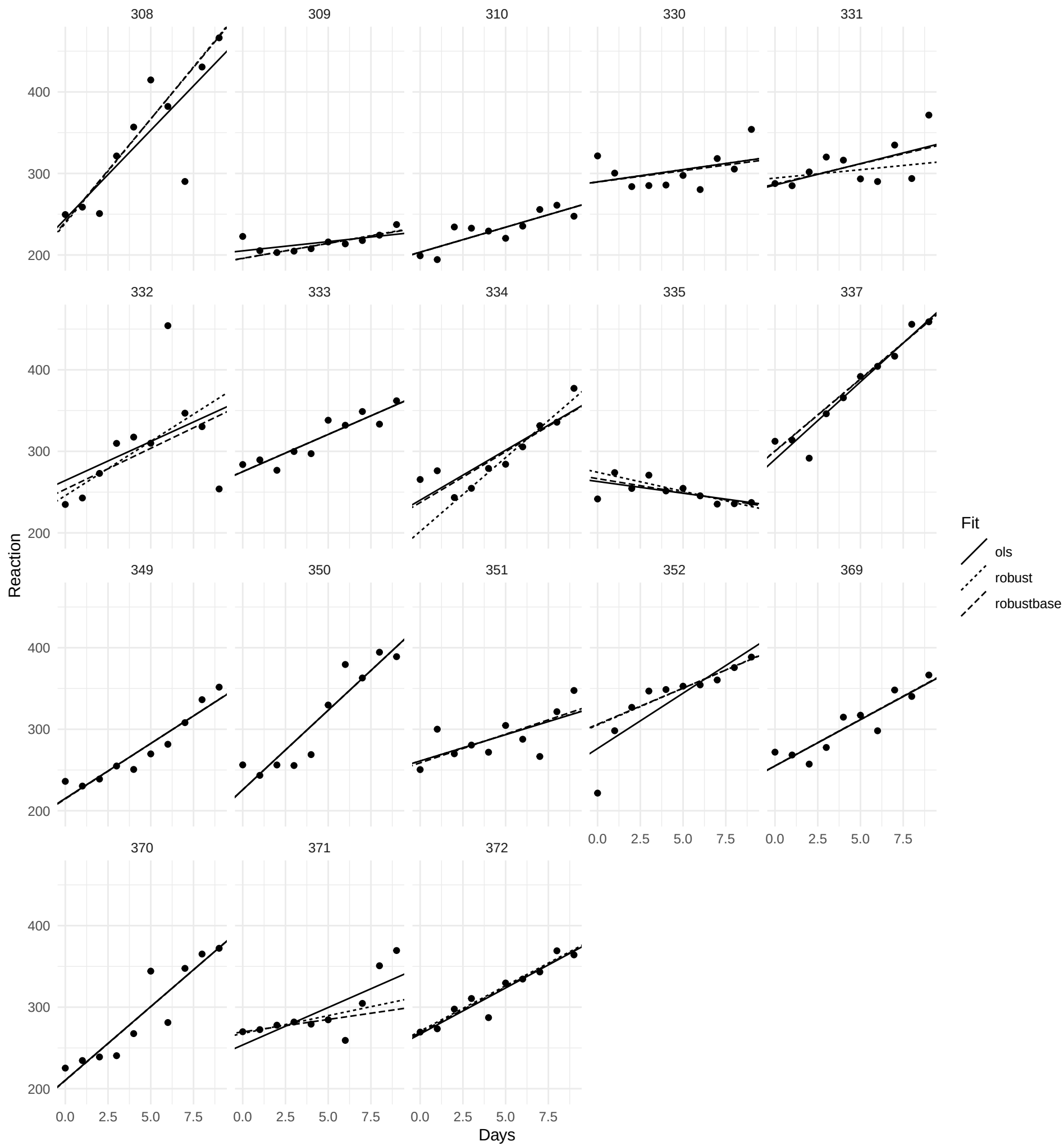
Selected within-cluster linear fits
