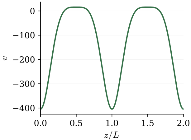
Kawahara elliptic wave: g_2 = 1 , g_3 = 0
