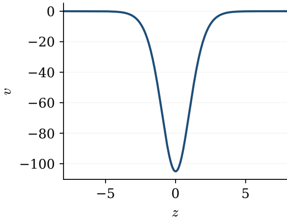
Kawahara solitary wave
