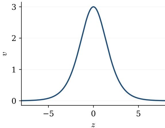
KdV soliton: P = D^2 - 1
