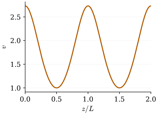
KdV cnoidal wave: P = D^2 - 1
