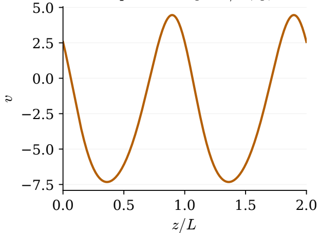
KS elliptic wave: g_2 = 1/12, g_3 = 0
