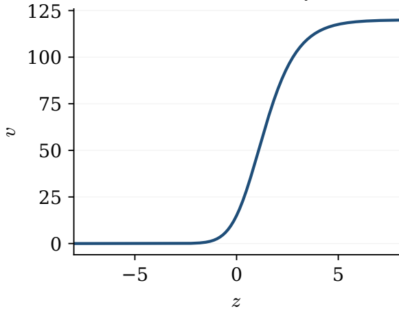
KS front: v = 120Q^3
