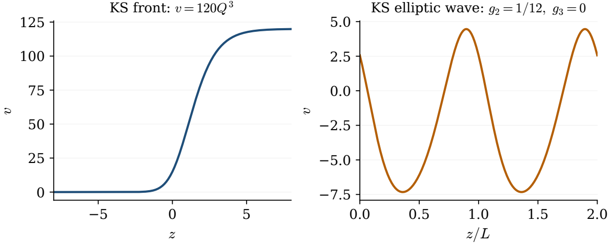
Figure 2: A KS front v = 120Q^3 and a bounded elliptic wave. For the latter, g_2 = 1/12 , g_3 = 0 , P = D^3 + 4D^2 + D + \sqrt{26} , and v = -60\wp' - 60\wp - 1 - \sqrt{26} , translated by the imaginary half-period; L = 2\sqrt{2\sqrt{3}} K(1/2) is its real period. The operators in the two panels are different.
