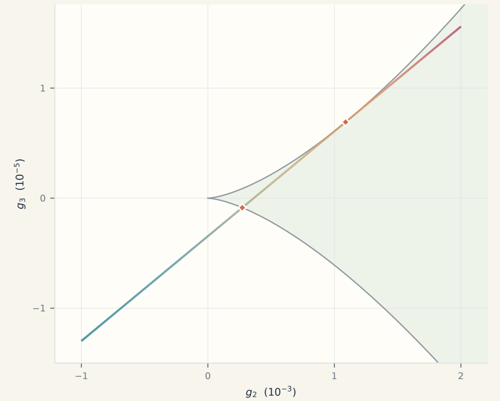
(7, 6) Septic
