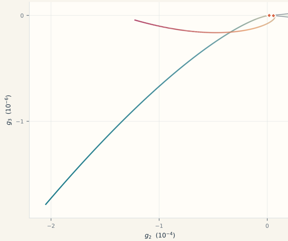
(2, 4) Kawahara-KS
