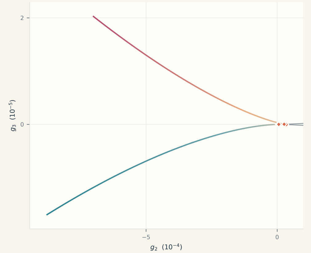
(3, 4) Swift-Hohenberg
