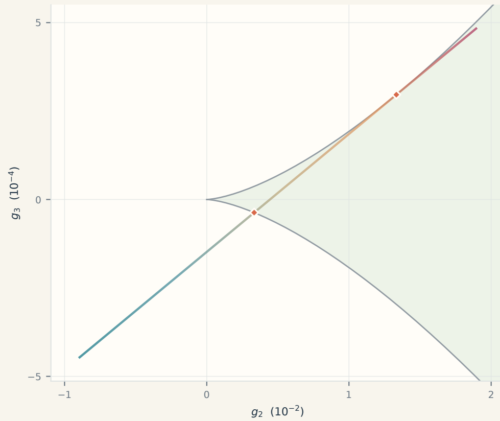
(5, 4) Quintic
