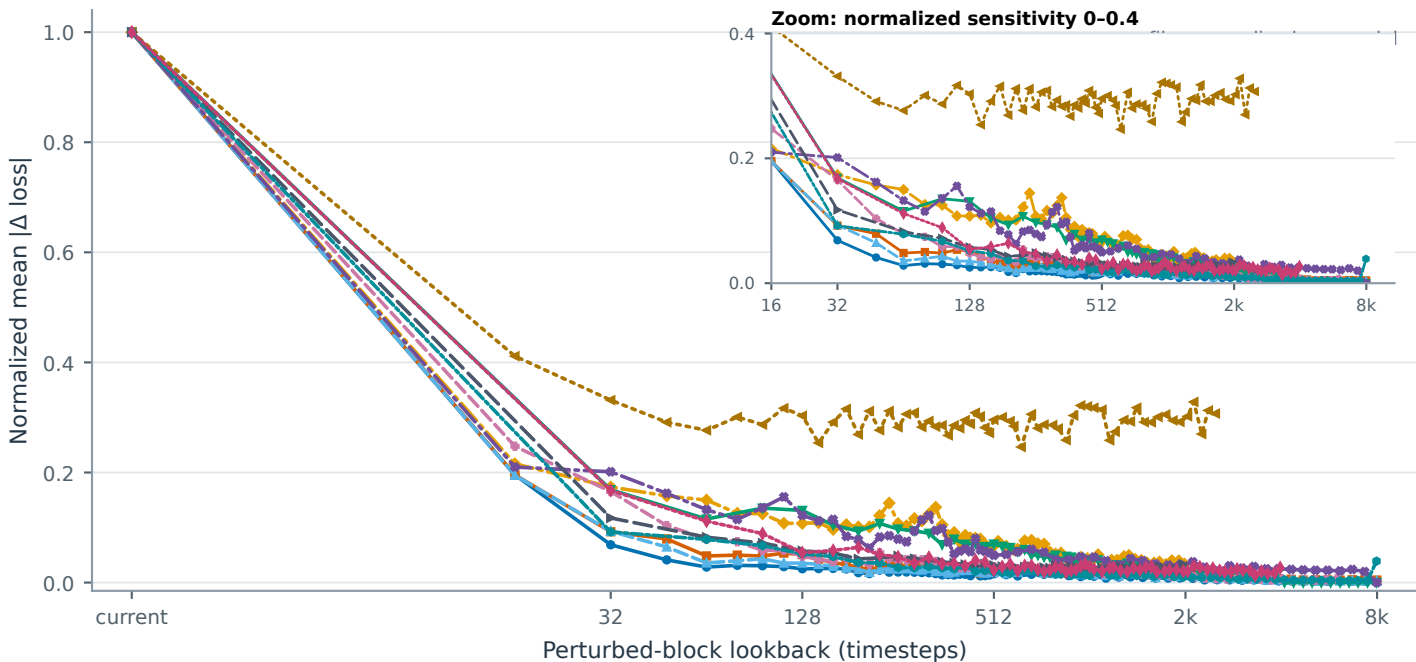
Block-mean perturbation sensitivity by lookback
