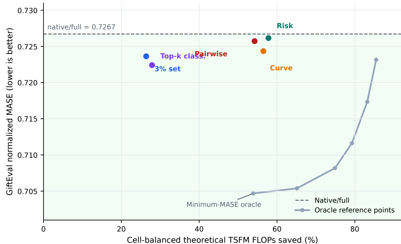
Synthetic-only selector operating points on Chronos2-Small
